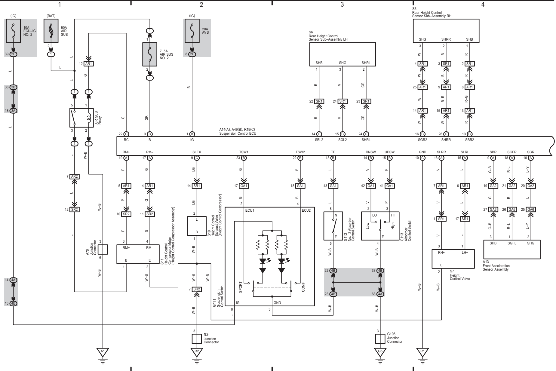
Electronic Modulated Air Suspension (RHD) (Before Aug. 2013 Production)
