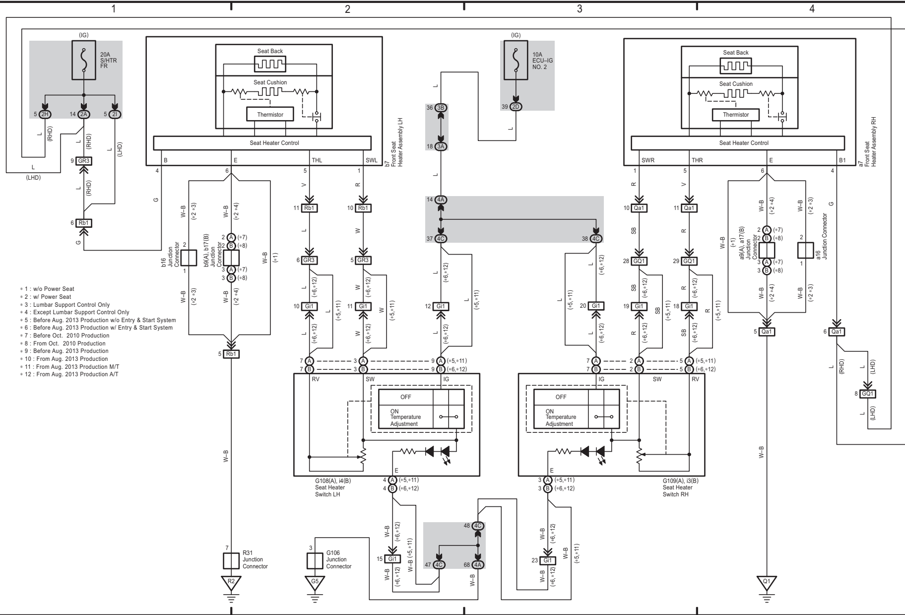
Seat Heater (Front) (Before Aug. 2017 Production)
