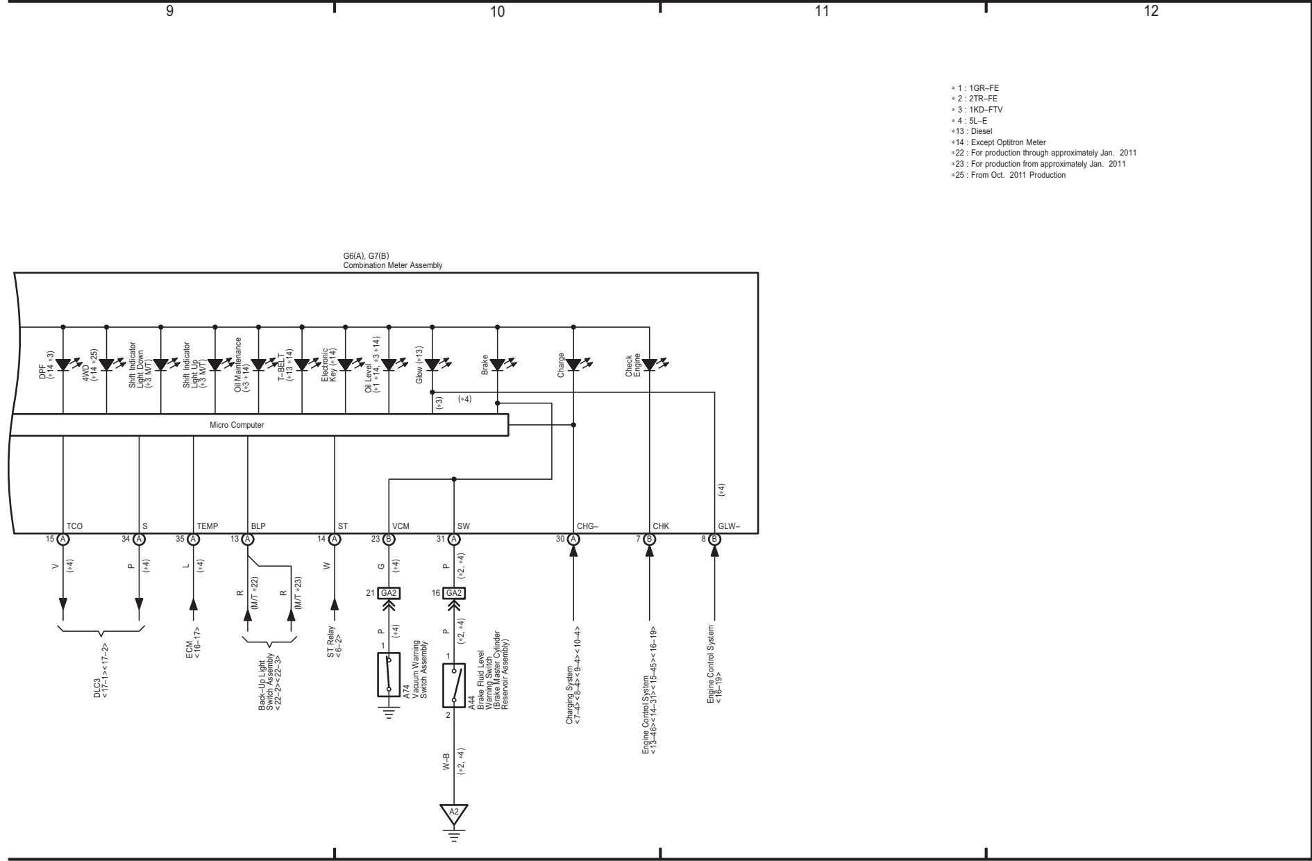
Combination Meter (LHD) (Before Aug. 2013 Production)
