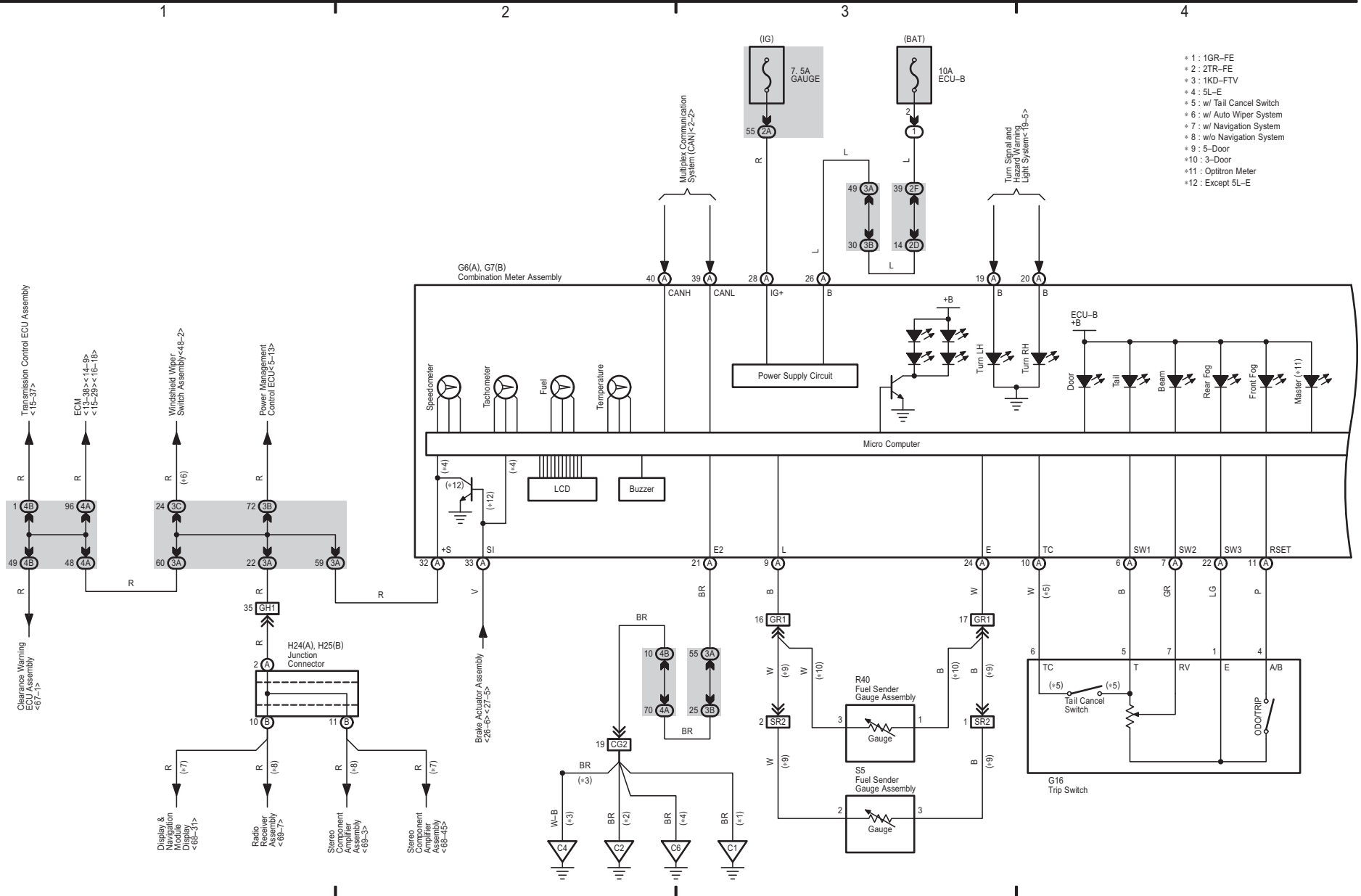
Combination Meter (LHD) (Before Aug. 2013 Production)
