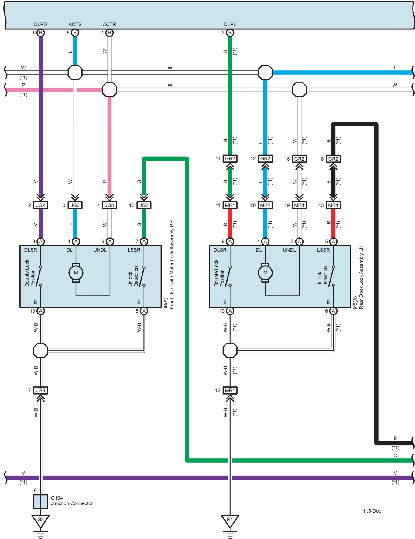
G212(B) Double Lock Door Control Relay Assembly
