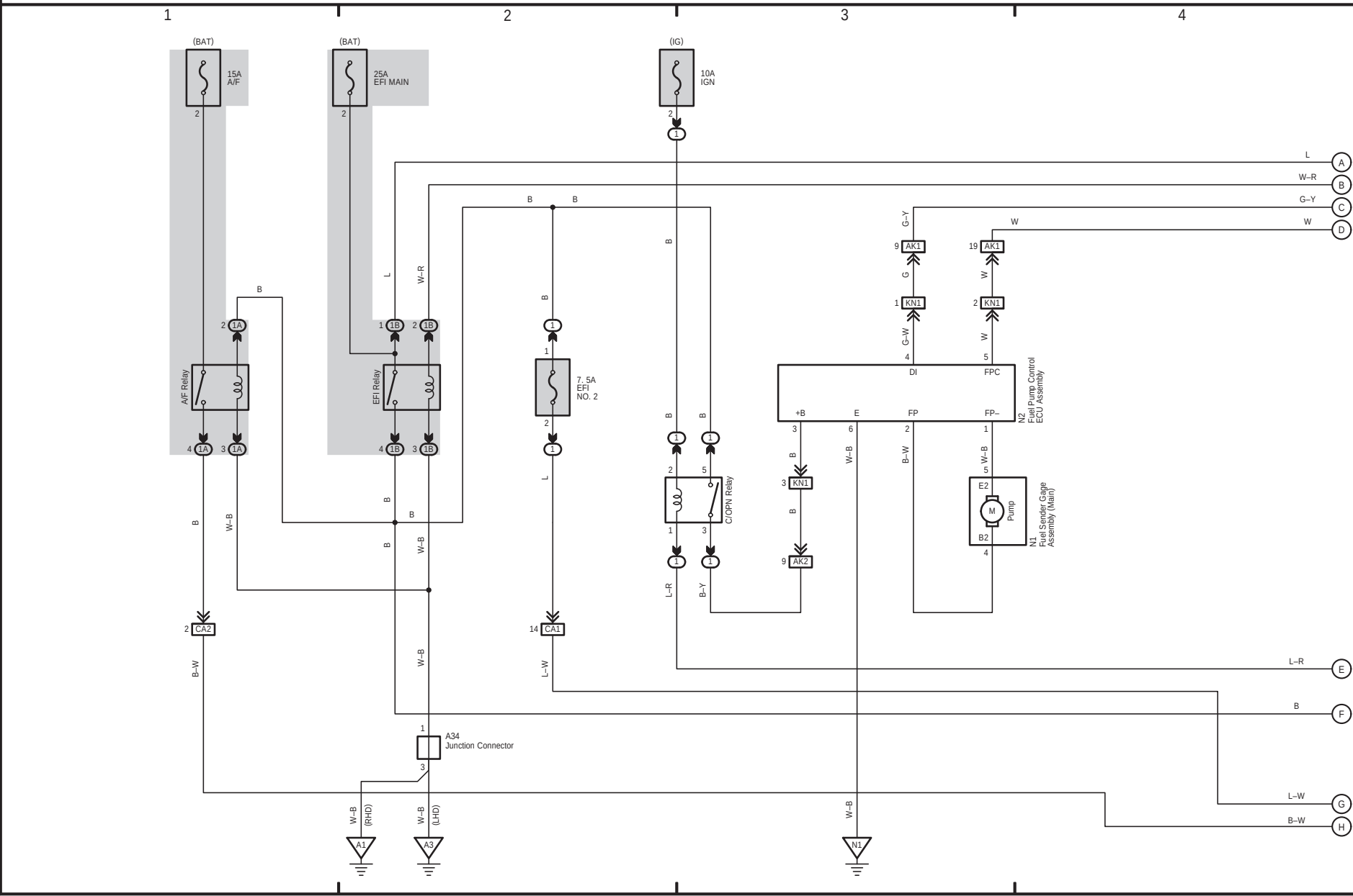
Engine Control (1GR-FE) (Before Jan. 2012 Production)
