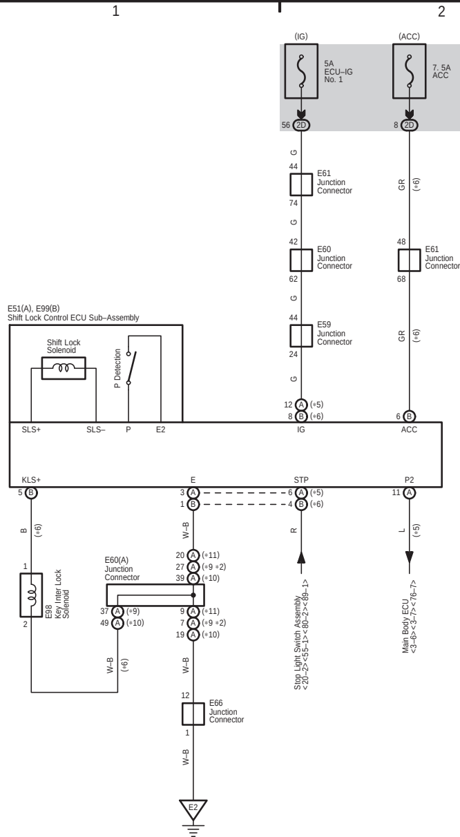
Shift Lock (Before Aug. 2015 Production)
