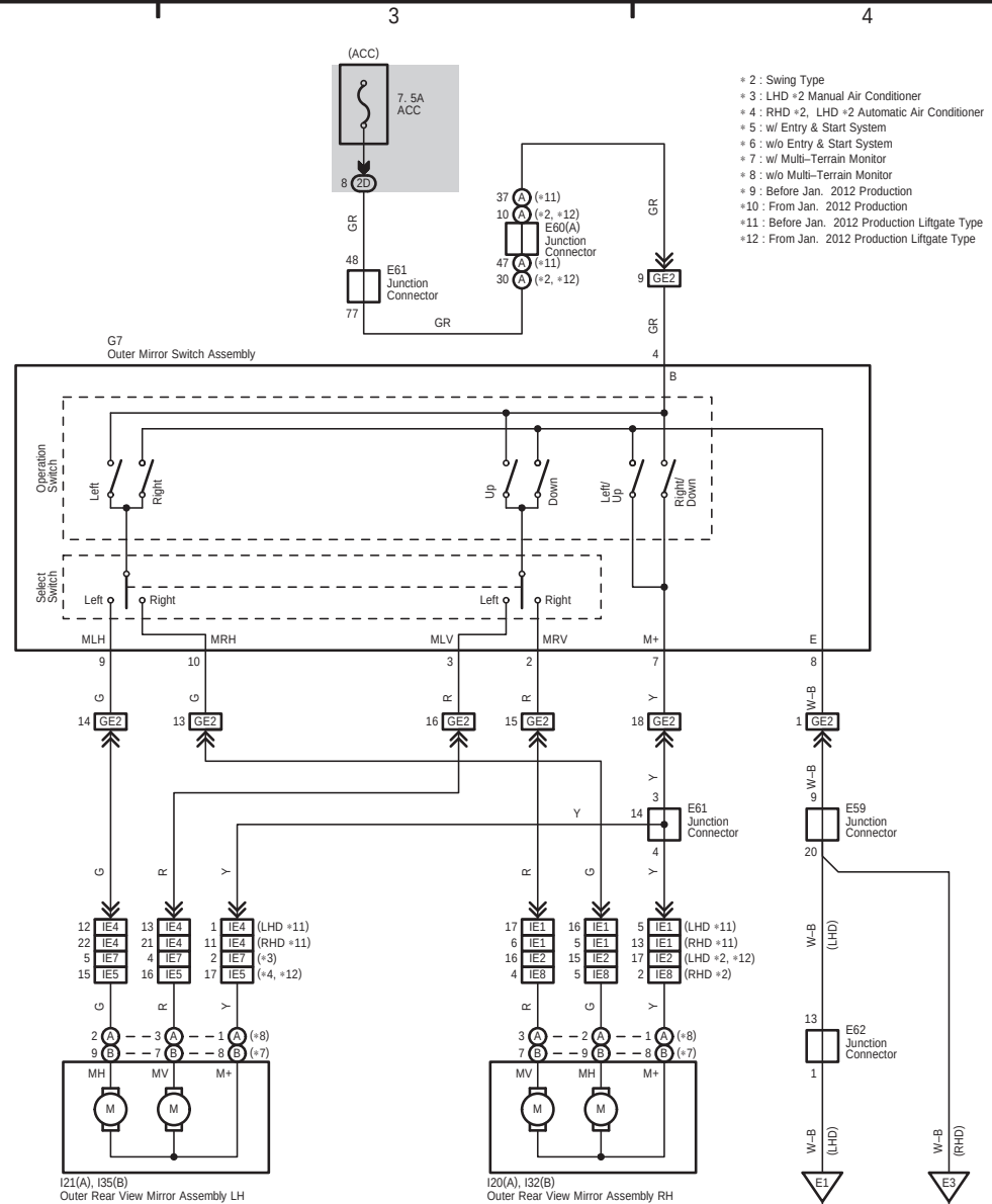
Remote Control Mirror (w/o Retractor) (Before Aug. 2015 Production)
