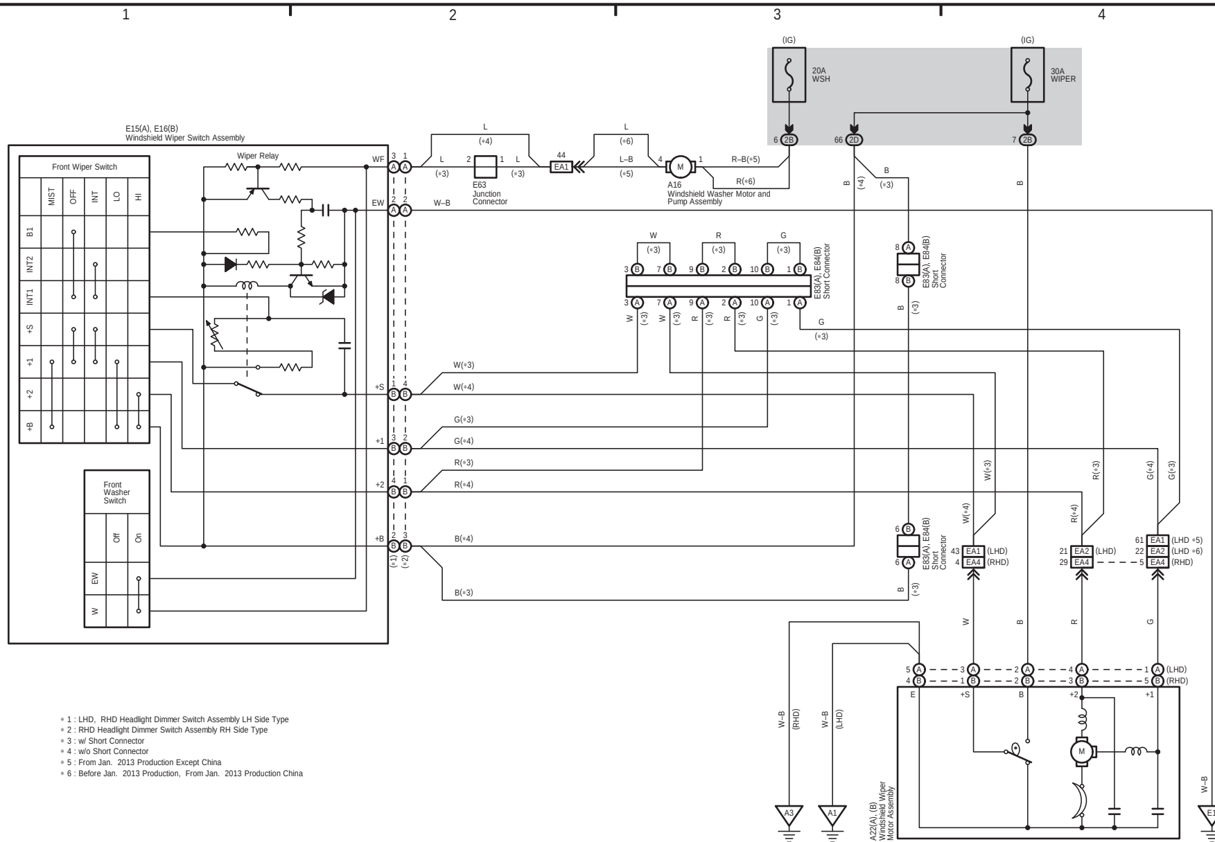
Front Wiper and Washer (w/o Auto Wiper System) (Before Aug. 2015 Production)
