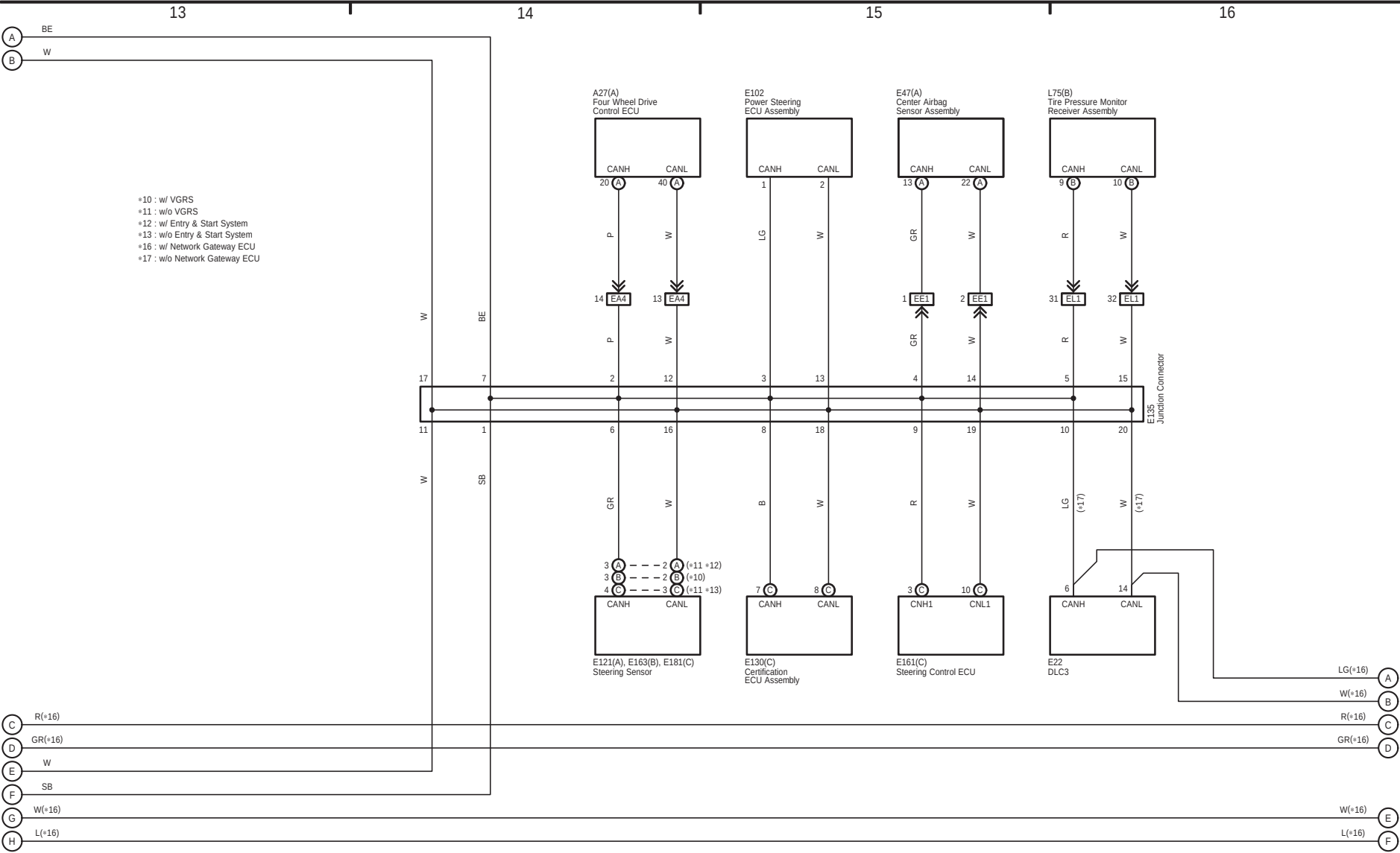
Multiplex Communication System (CAN RHD) (From Aug. 2015 Production)
