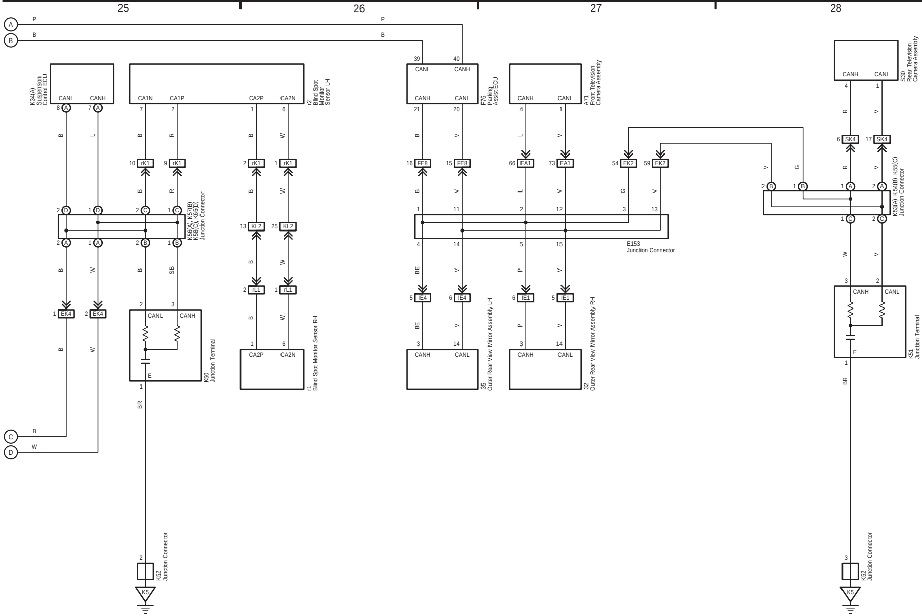
Multiplex Communication System (CAN RHD) (From Aug. 2015 Production)
