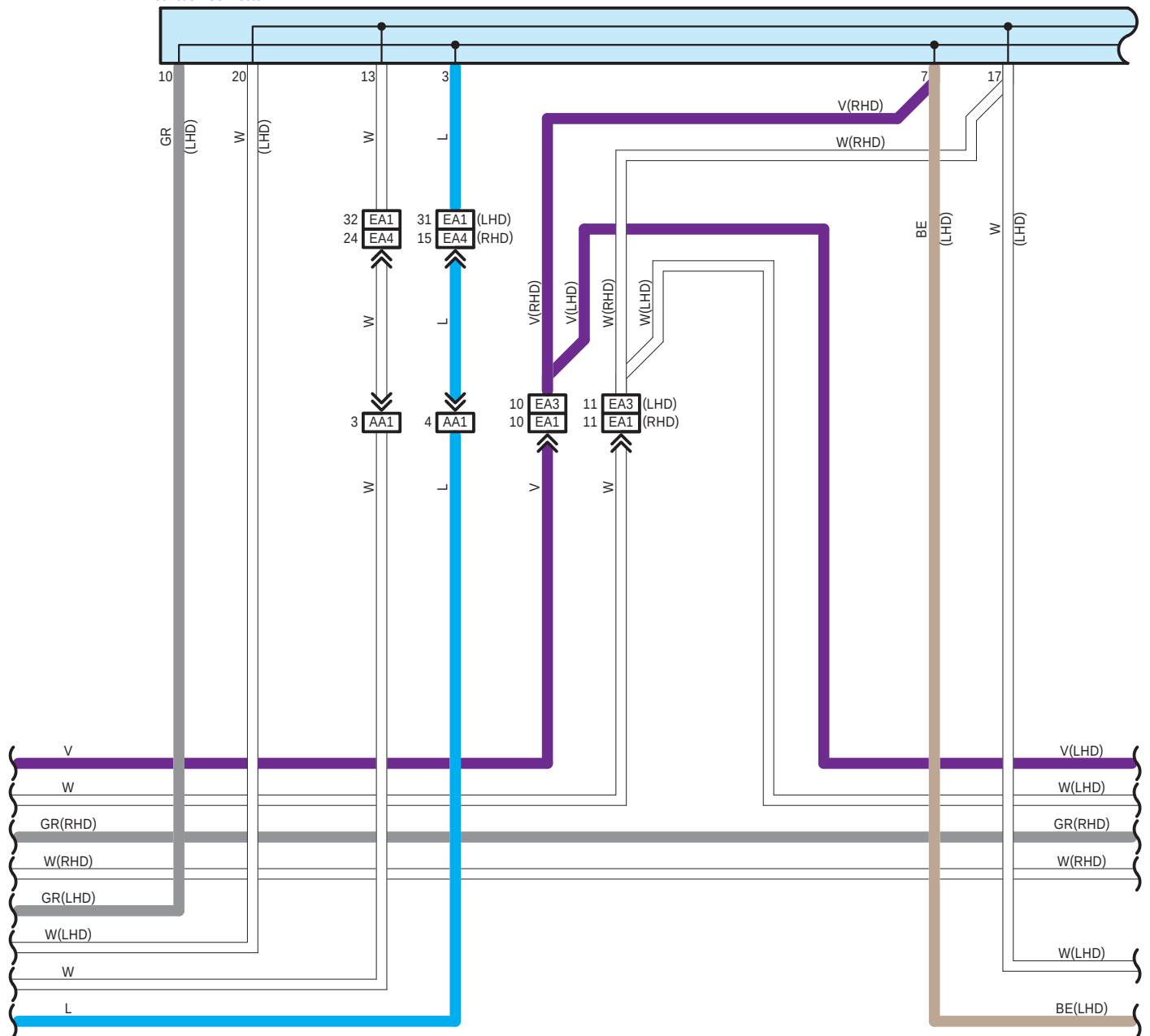
E133 Junction Connector
