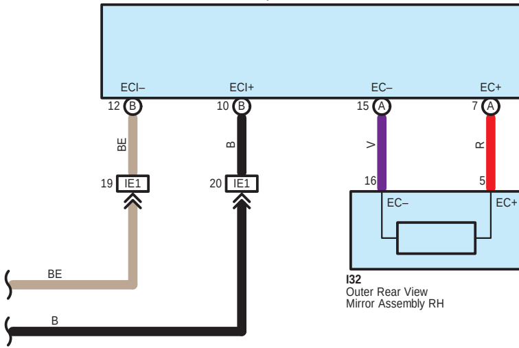
I37(A), I38(B) Outer Mirror Control ECU Assembly RH
