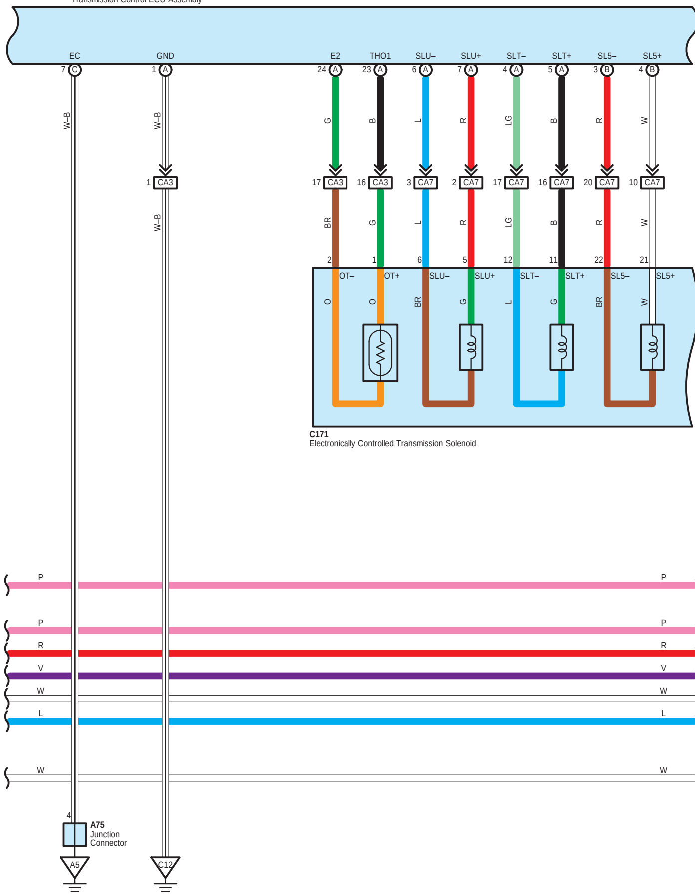
A80(A), A81(B), A82(C) Transmission Control ECU Assembly
