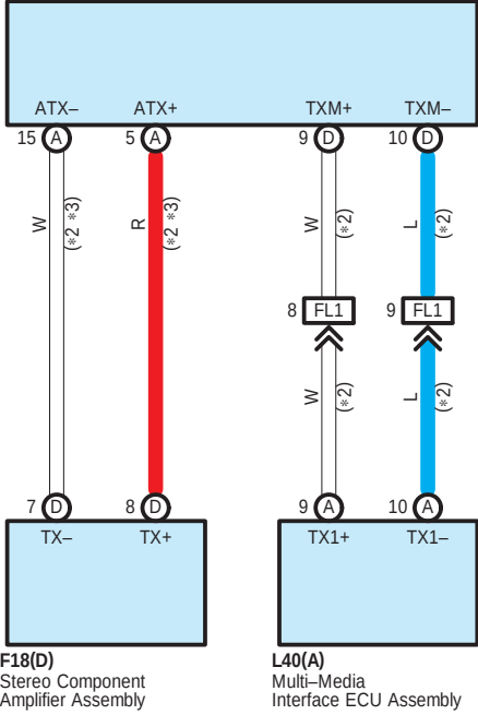
F1(A), F55(D) Radio Receiver Assembly
