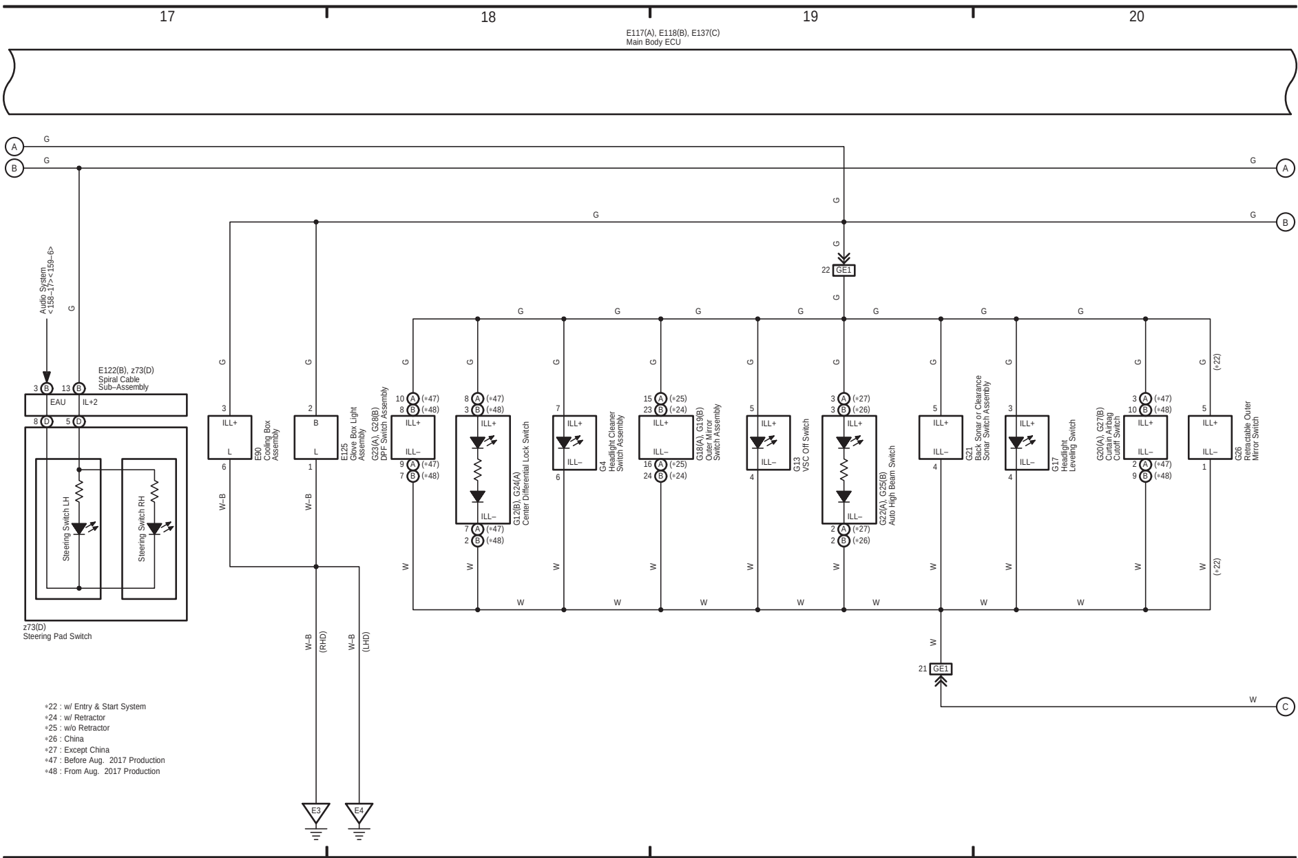
Taillight (From Aug. 2015 Production)
