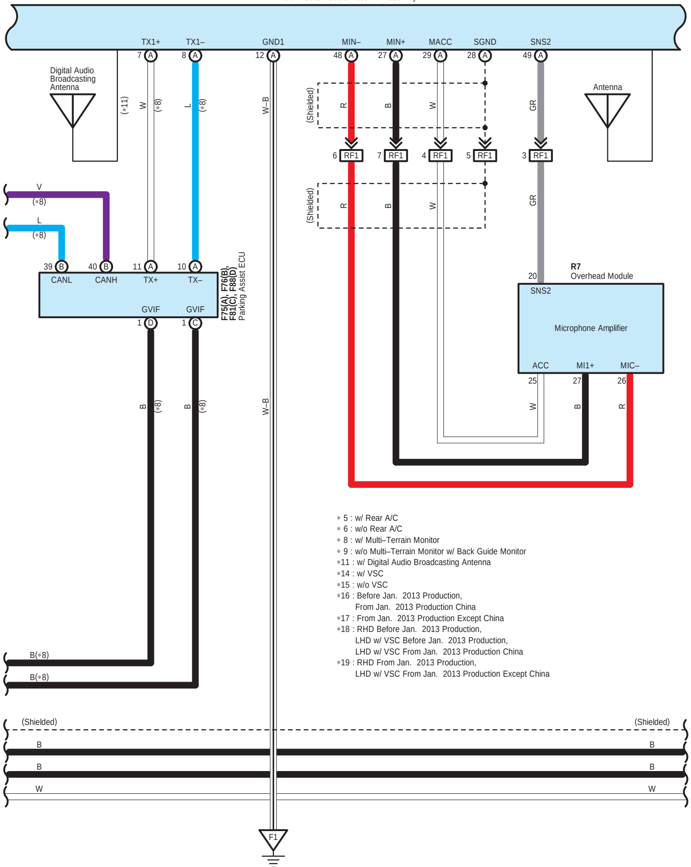
F77(A), F78(B), F82(C), F84(D), F86(E) Multi-Media Module Receiver Assembly
