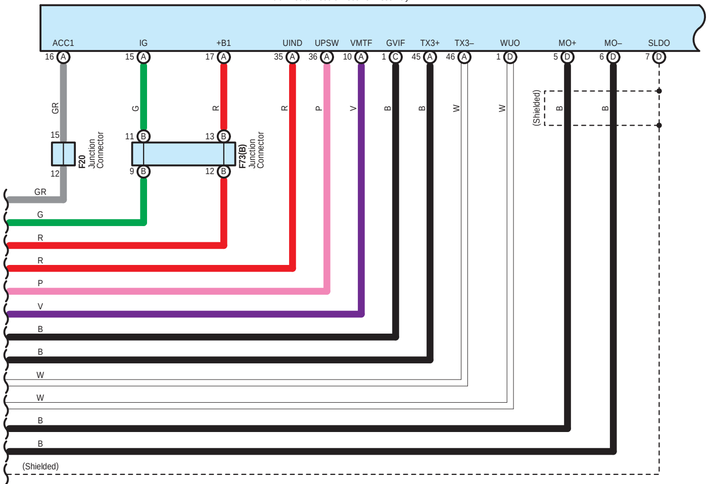
F77(A), F78(B), F82(C), F84(D), F86(E) Multi-Media Module Receiver Assembly
