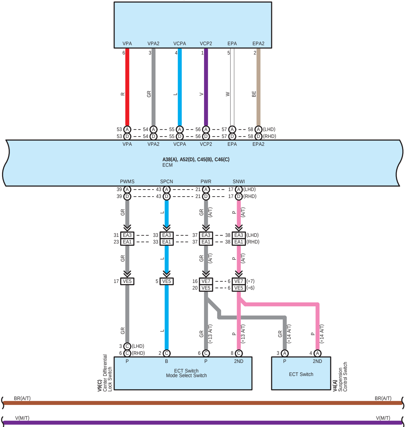
A31 Accelerator Pedal Sensor Assembly
