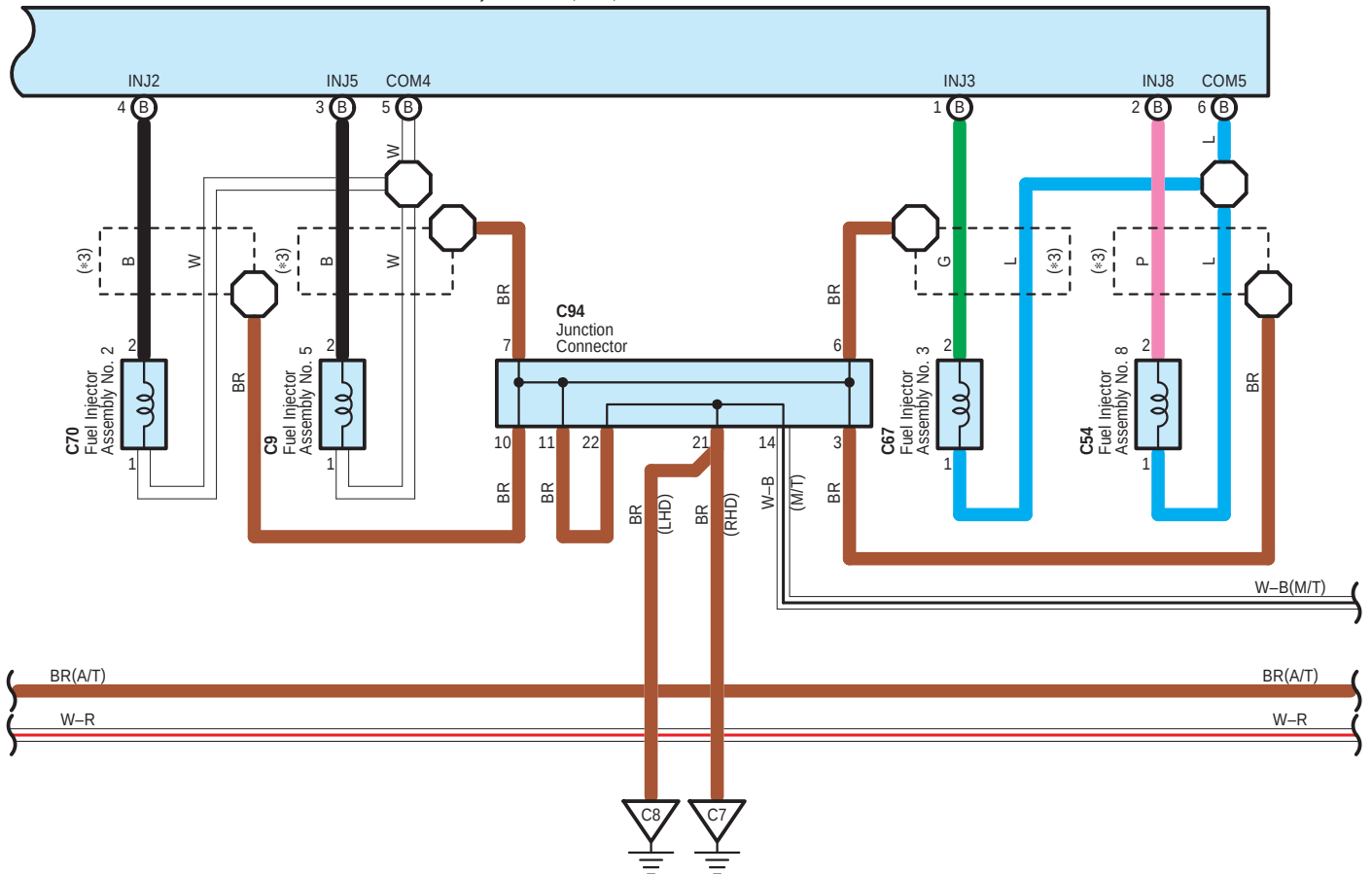
C75(A), C76(B) Injector Driver (No. 2)
