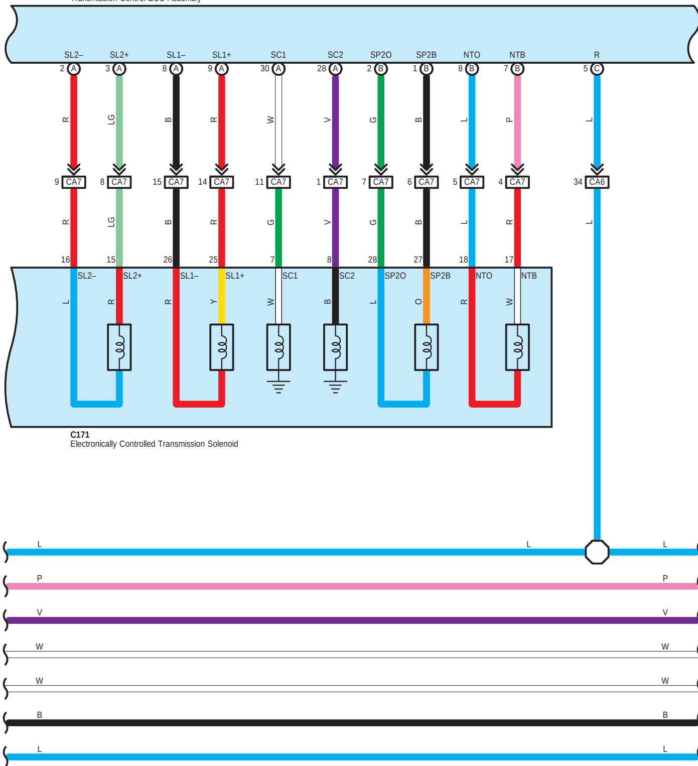
A80(A), A81(B), A82(C) Transmission Control ECU Assembly
