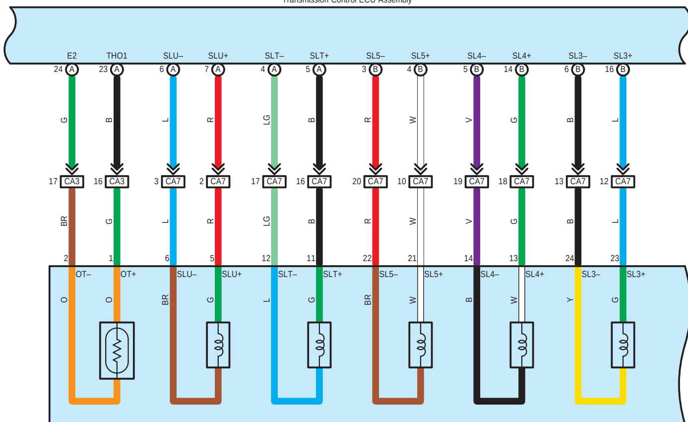
C171 Electronically Controlled Transmission Solenoid
