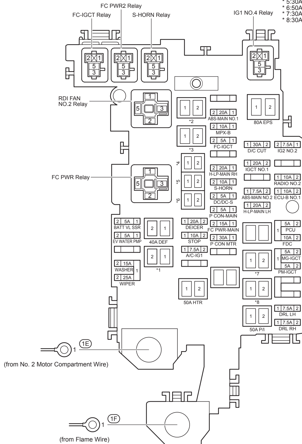
Top View
