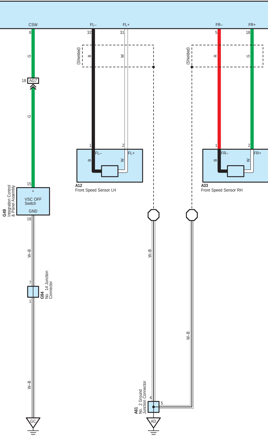
A63 Skid Control ECU Assembly
