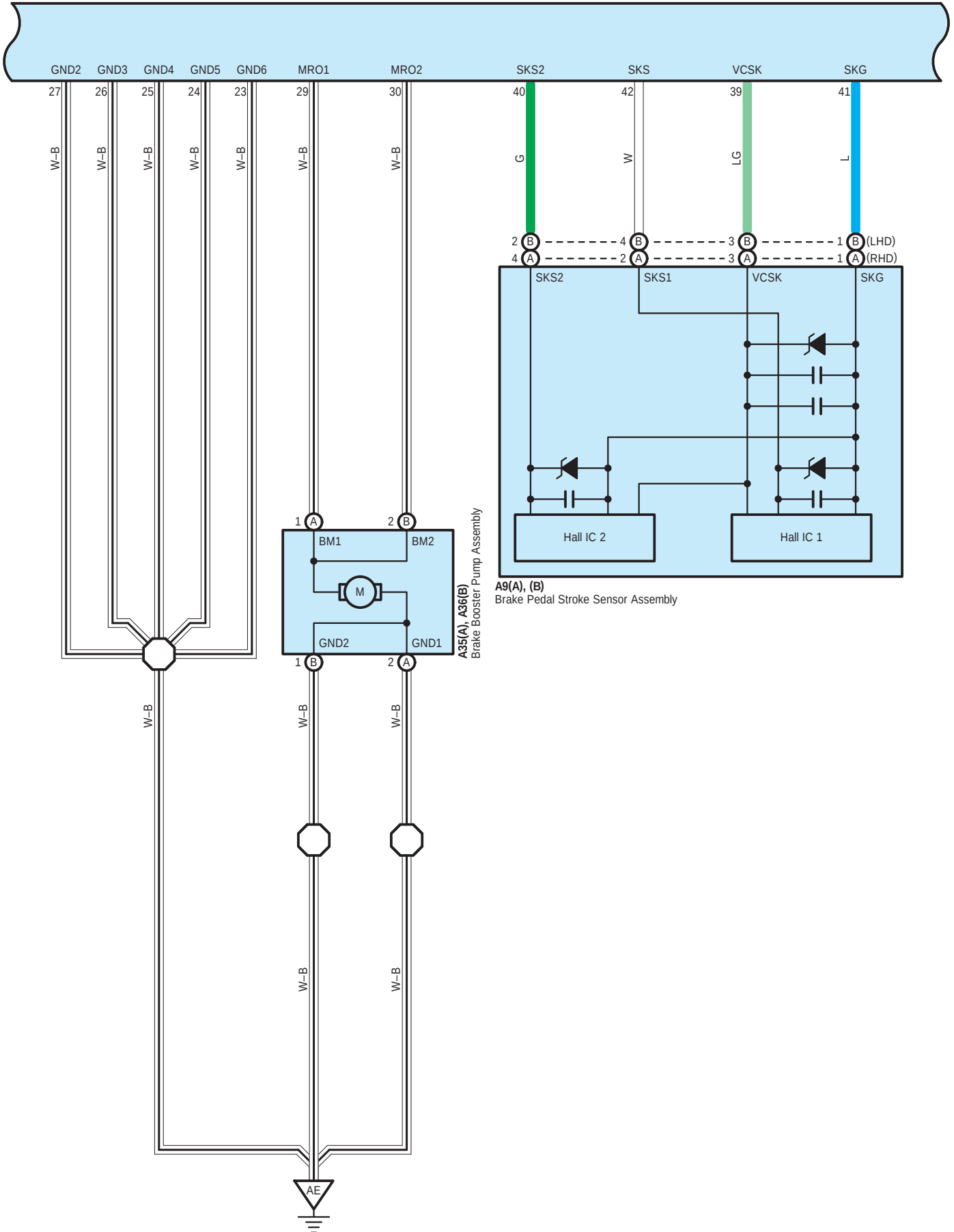
A63 Skid Control ECU Assembly
