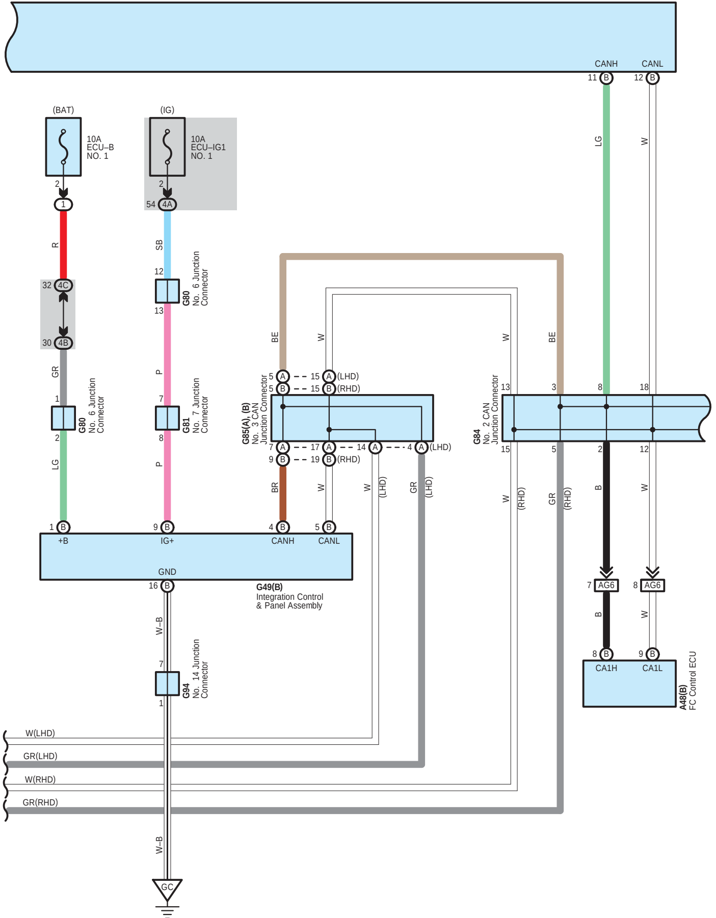
G42(A), G43(B), z1(C) Air Conditioning Amplifier Assembly
