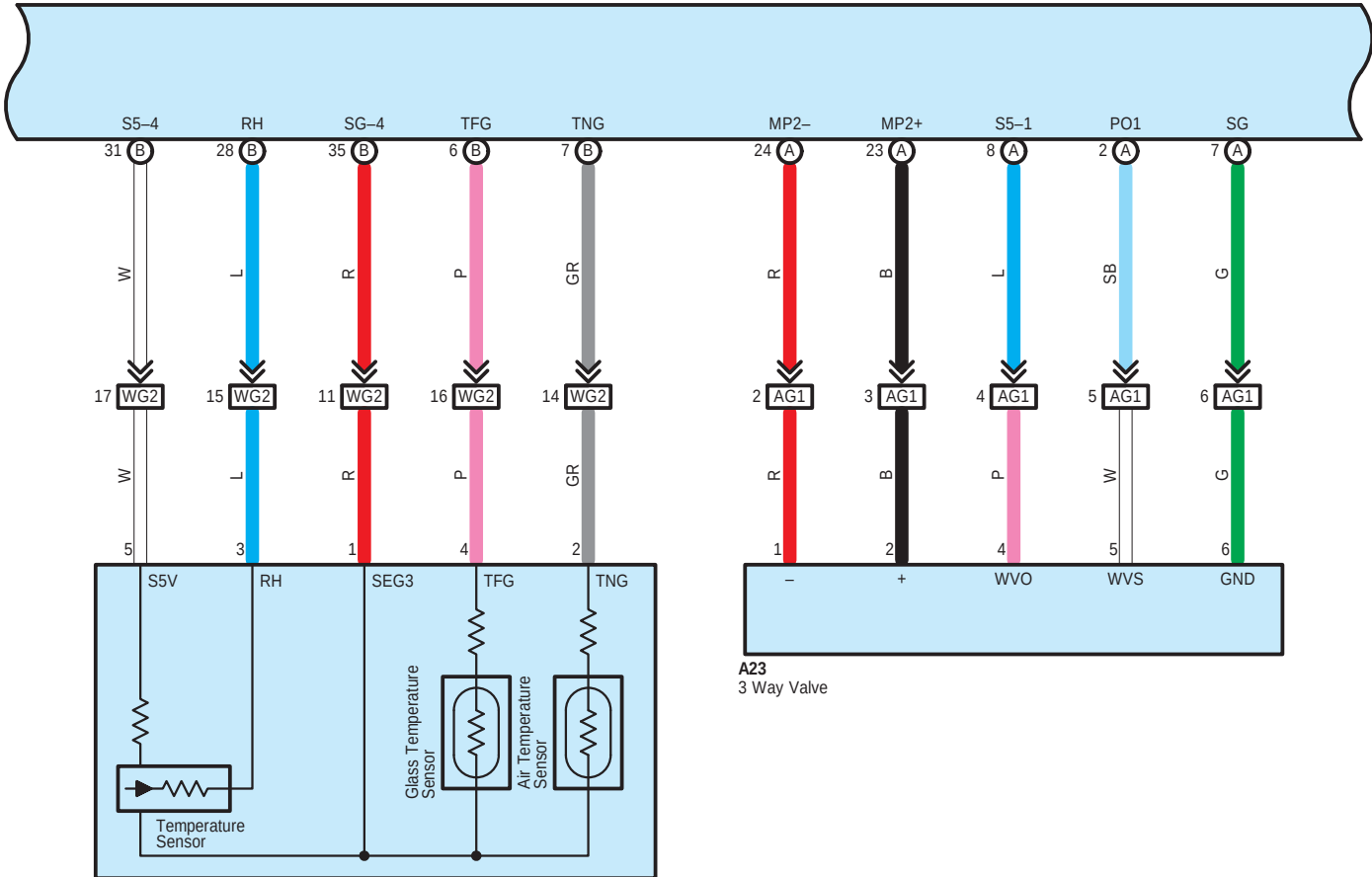
W11 Air Conditioning Thermistor Assembly
