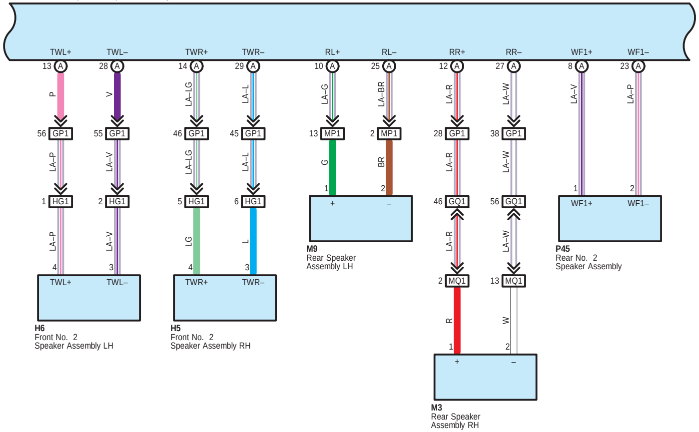
P48(A), P49(B) Stereo Component Amplifier Assembly
