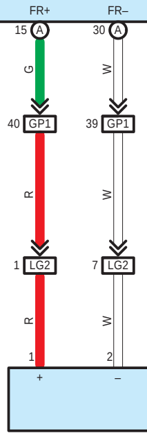
L2 Front No. 1 Speaker Assembly RH
