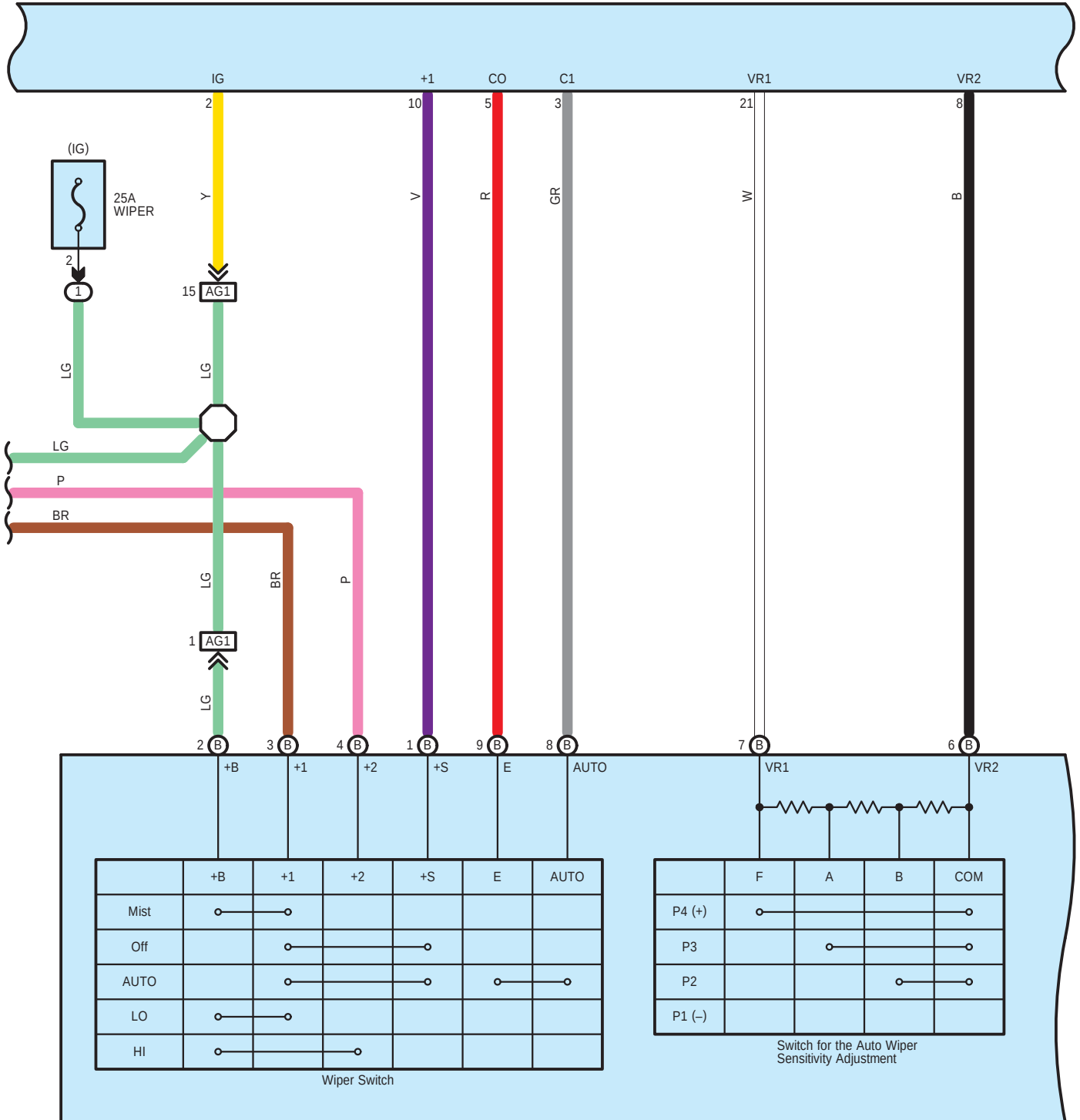
G26(A), G27(B) Windshield Wiper Switch Assembly
