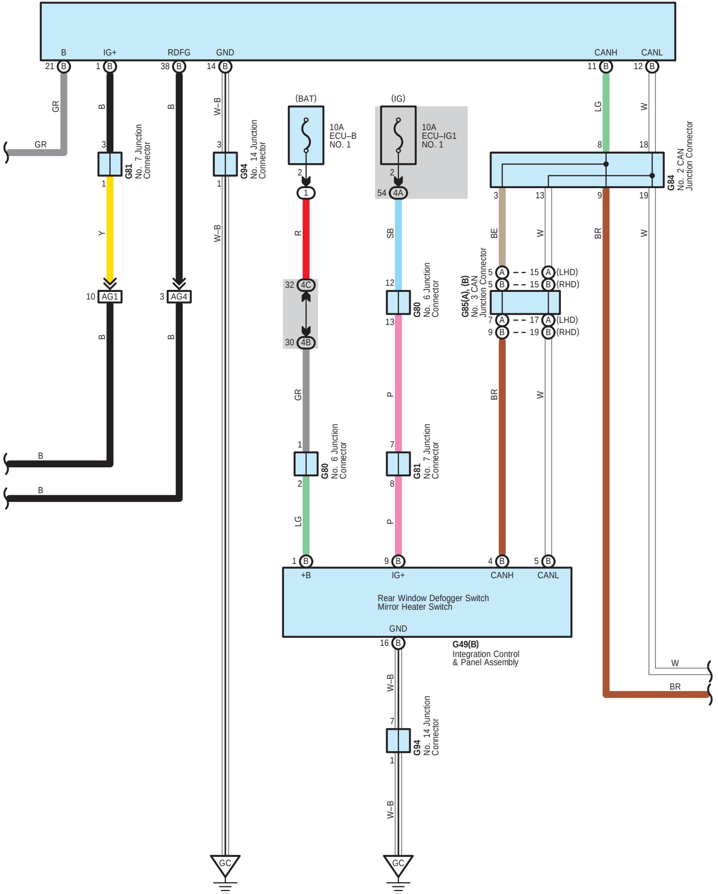
G43(B) Air Conditioning Amplifier Assembly
