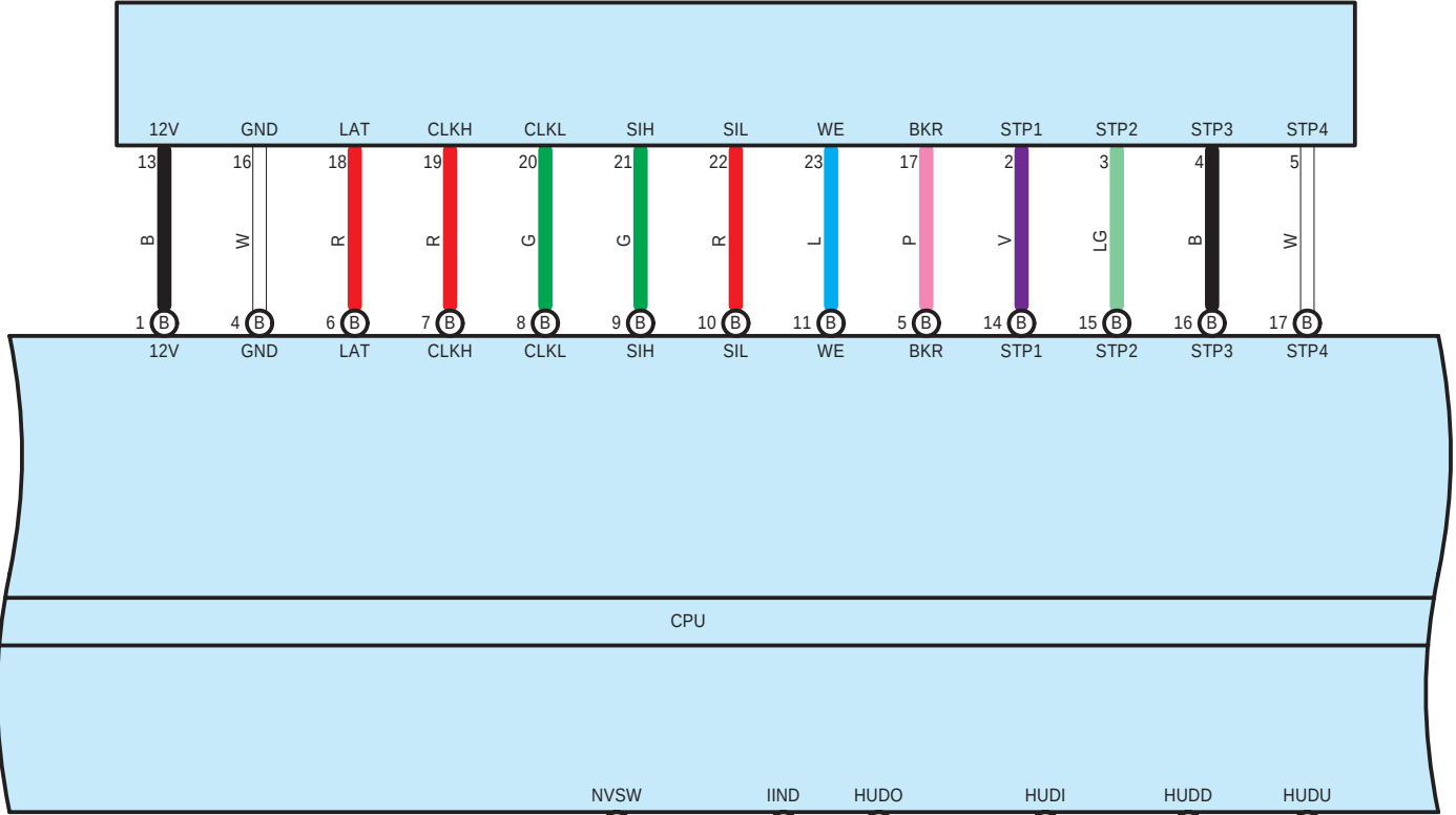
L27(A), L106(B), L107(C) Combination Meter Assembly
