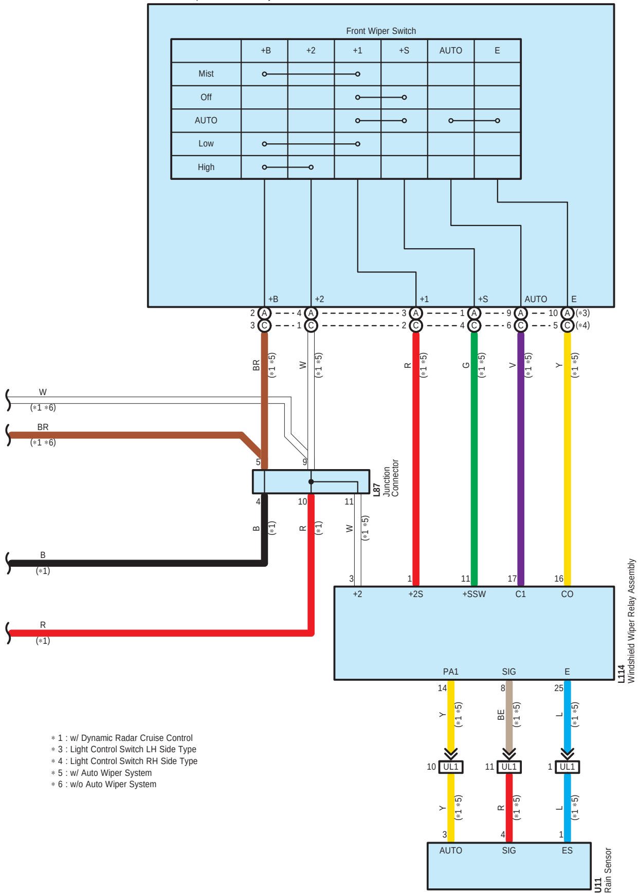
L48(A), (C) Windshield Wiper Switch Assembly
