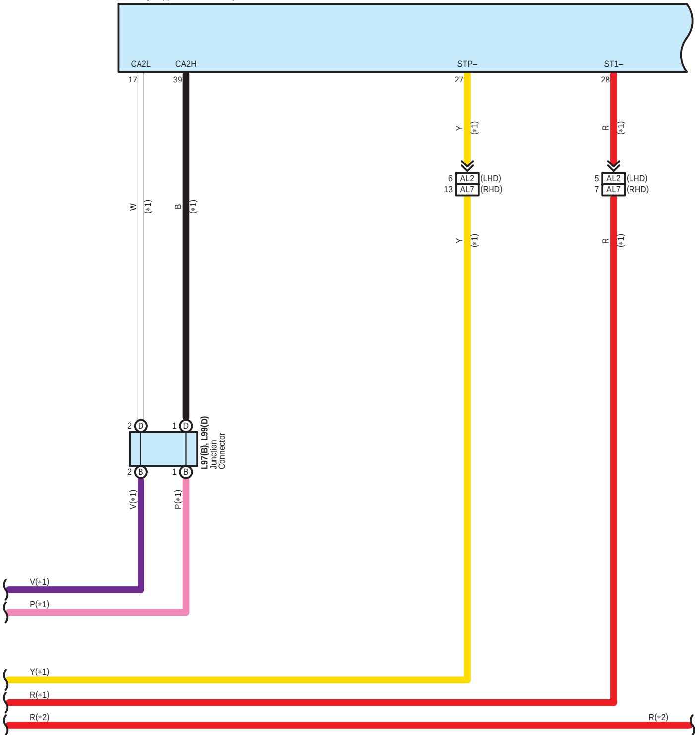
L60 Driving Support ECU Assembly
