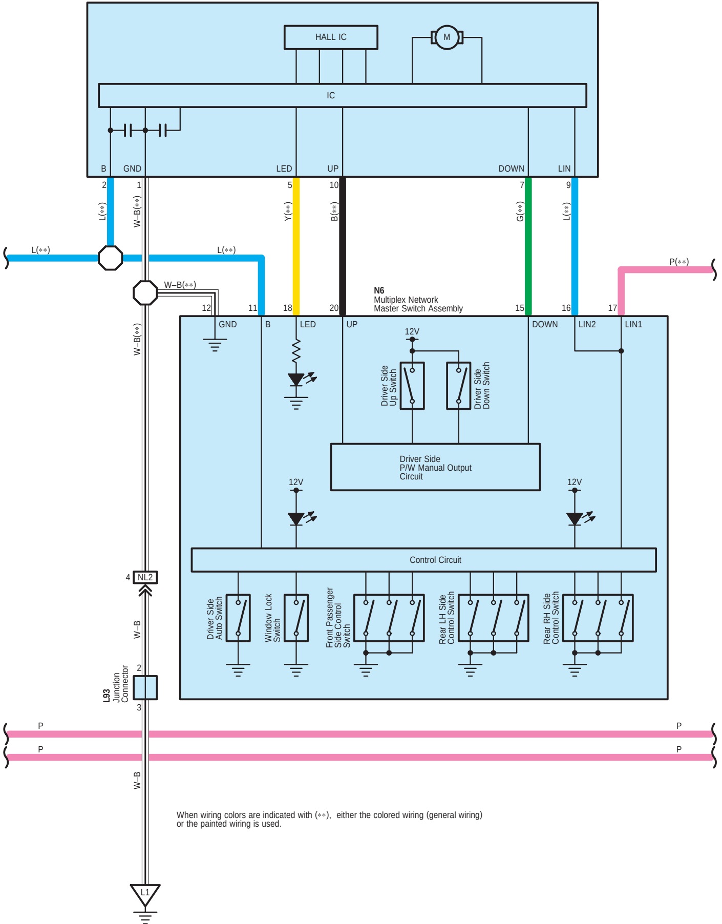
N2 Front Power Window Regulator Motor Assembly RH
