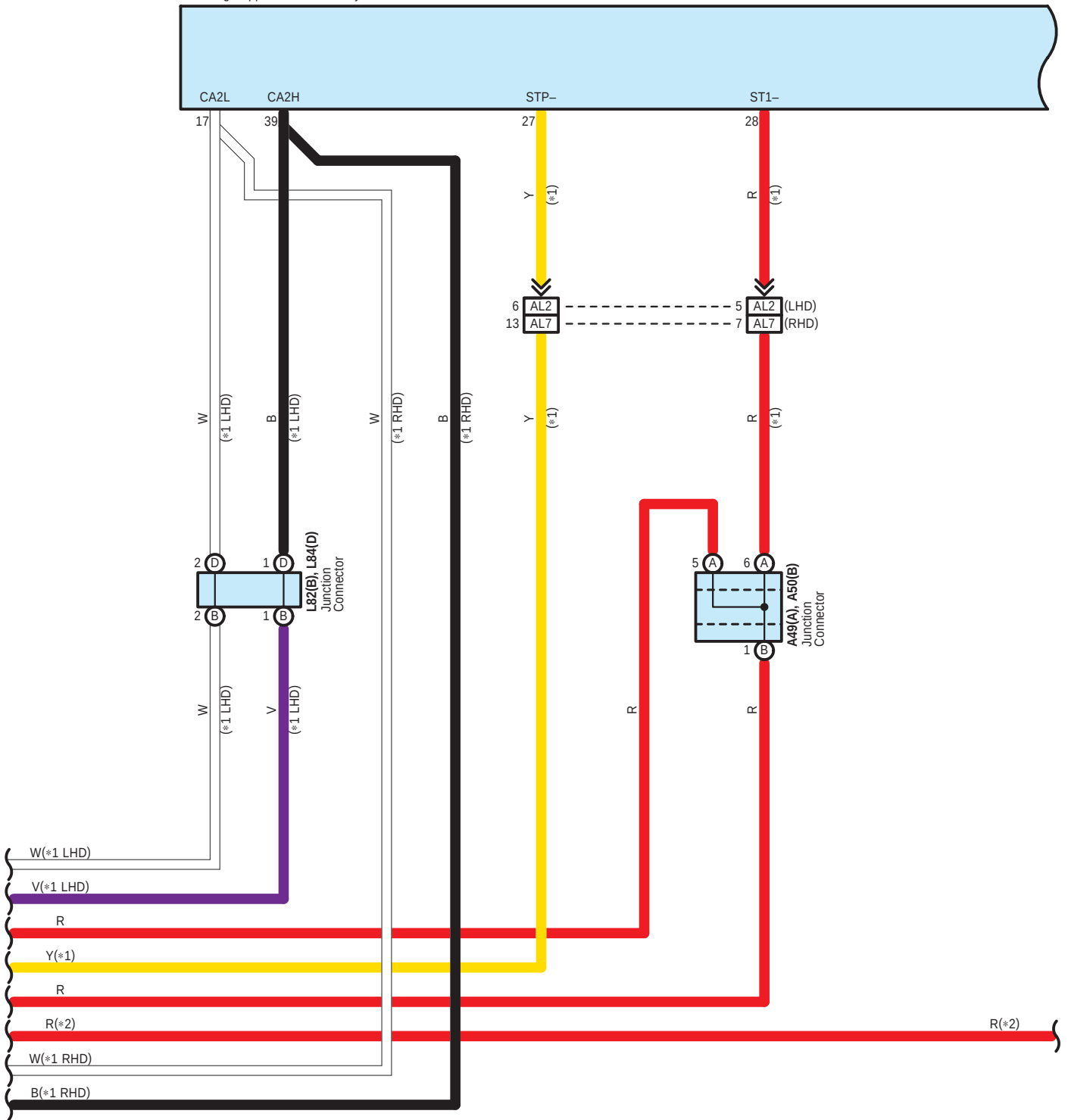
L54 Driving Support ECU Assembly
