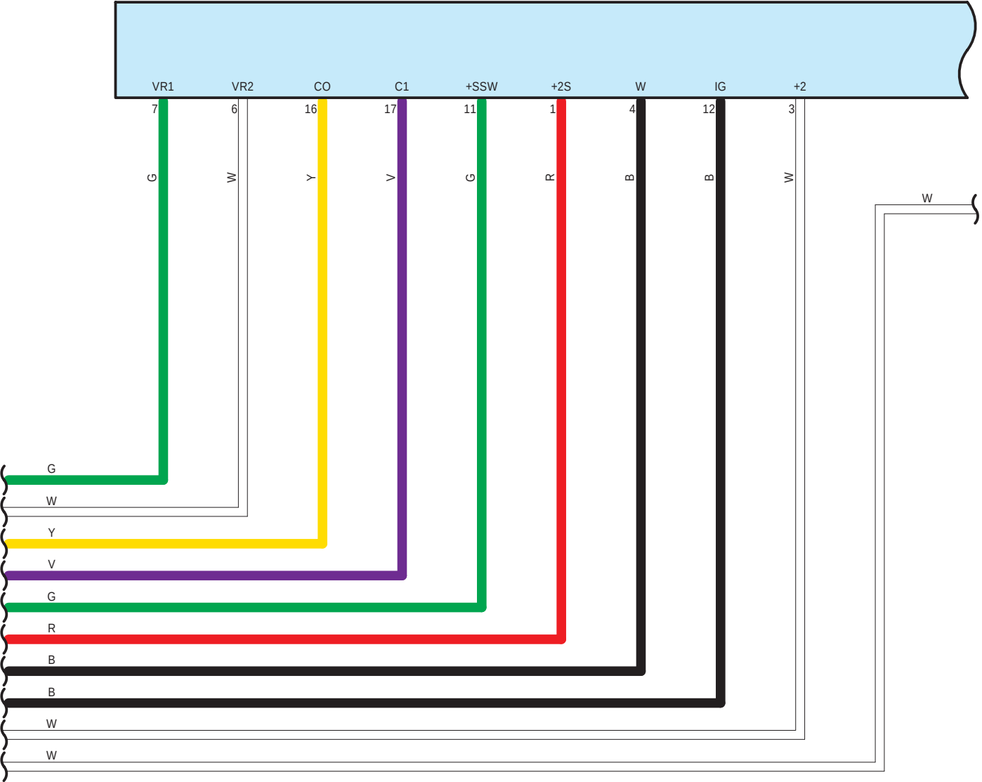
L63 Windshield Wiper Relay Assembly
