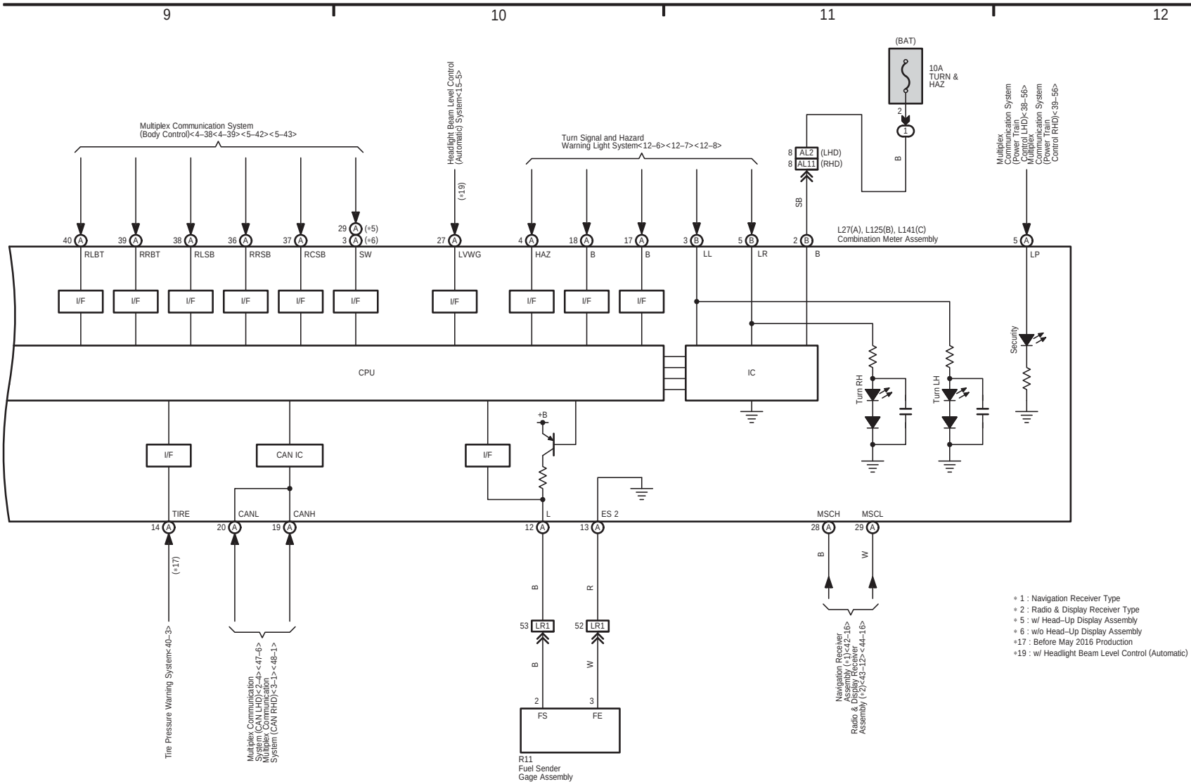
Combination Meter (From Nov. 2014 Production) and Headup Display (From Nov. 2014 Production)
