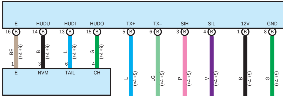
L147 Head-Up Display Switch Assembly
