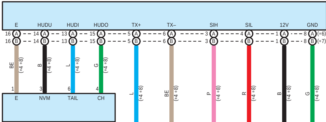
L147 Head-Up Display Switch Assembly
