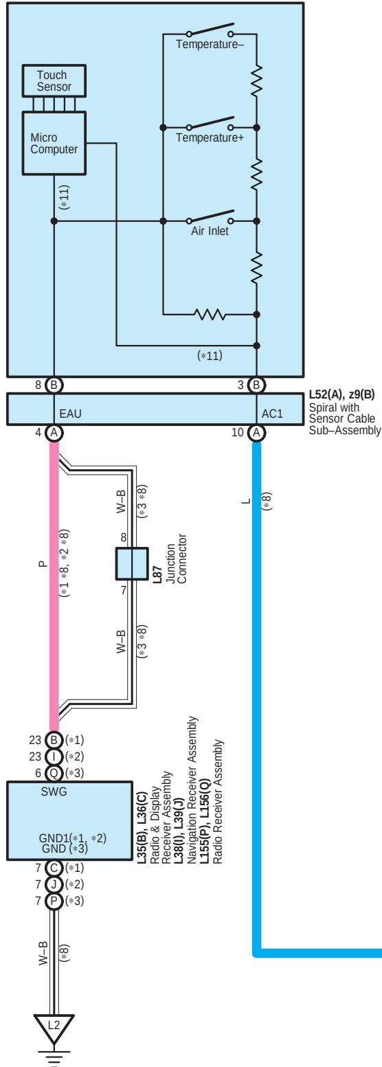
z9(B) Steering Pad Switch Assembly
