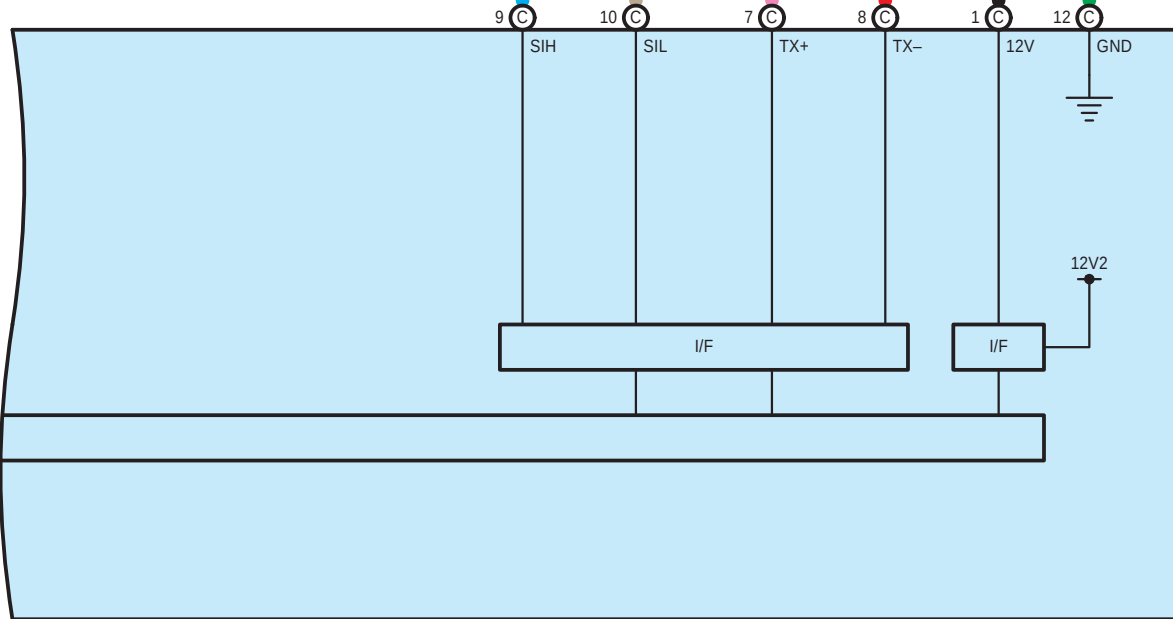
L27(A), L141(C) Combination Meter Assembly
