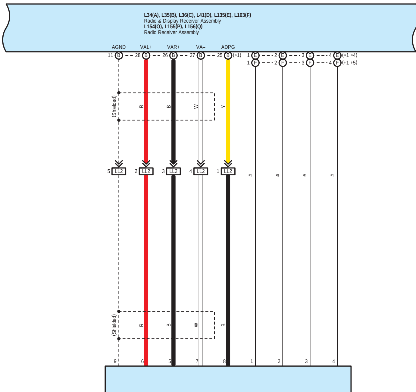
L13 No. 1 Stereo Jack Adapter Assembly
