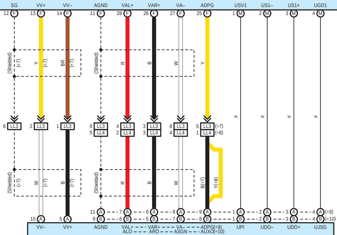
L174(A), L193(B) No. 1 Stereo Jack Adapter Assembly
