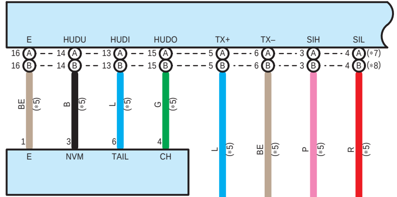
L147 Head-Up Display Switch Assembly
