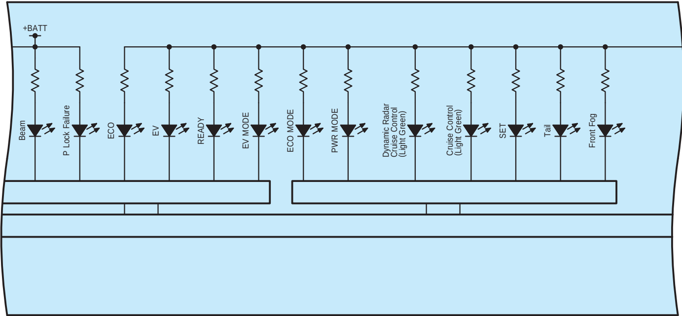
L27(A), L125(B), L141(C) Combination Meter Assembly
