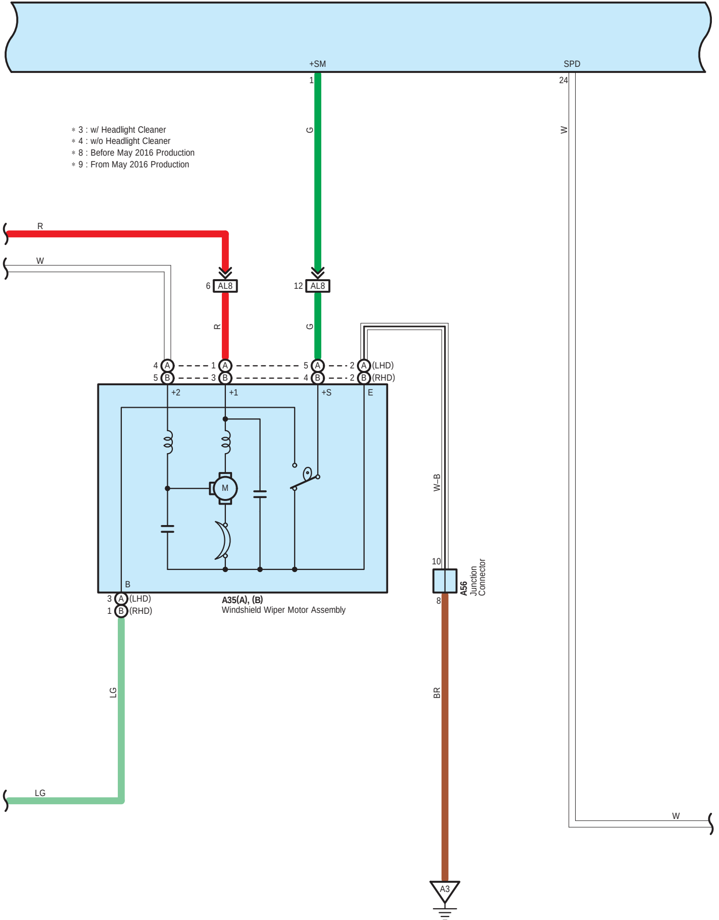
L146 Windshield Wiper Relay Assembly
