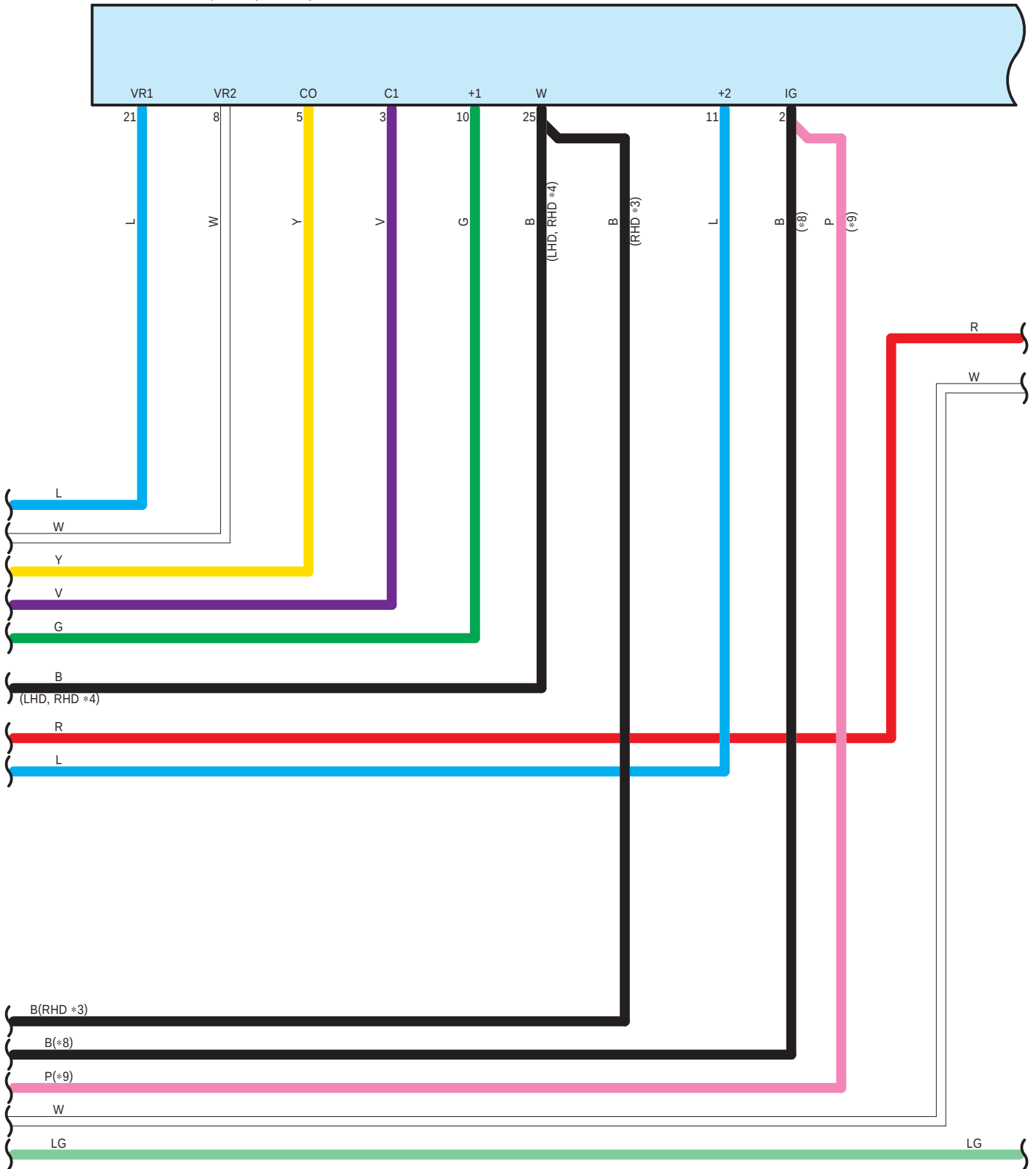
L146 Windshield Wiper Relay Assembly
