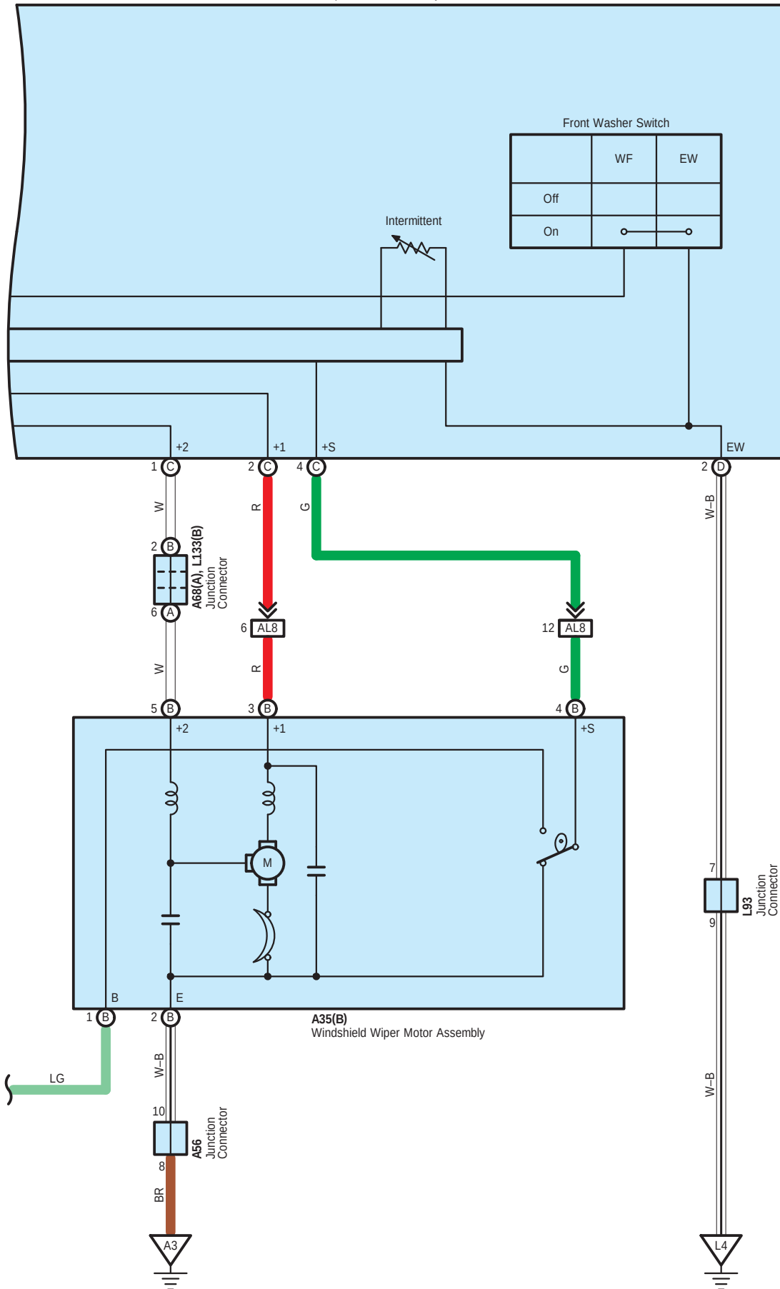
L48(C), L49(D) Windshield Wiper Switch Assembly
