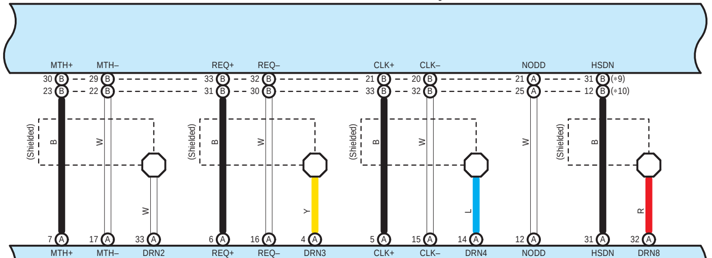
A21(A), A22(B), L5(C), L6(D) Power Management Control ECU
