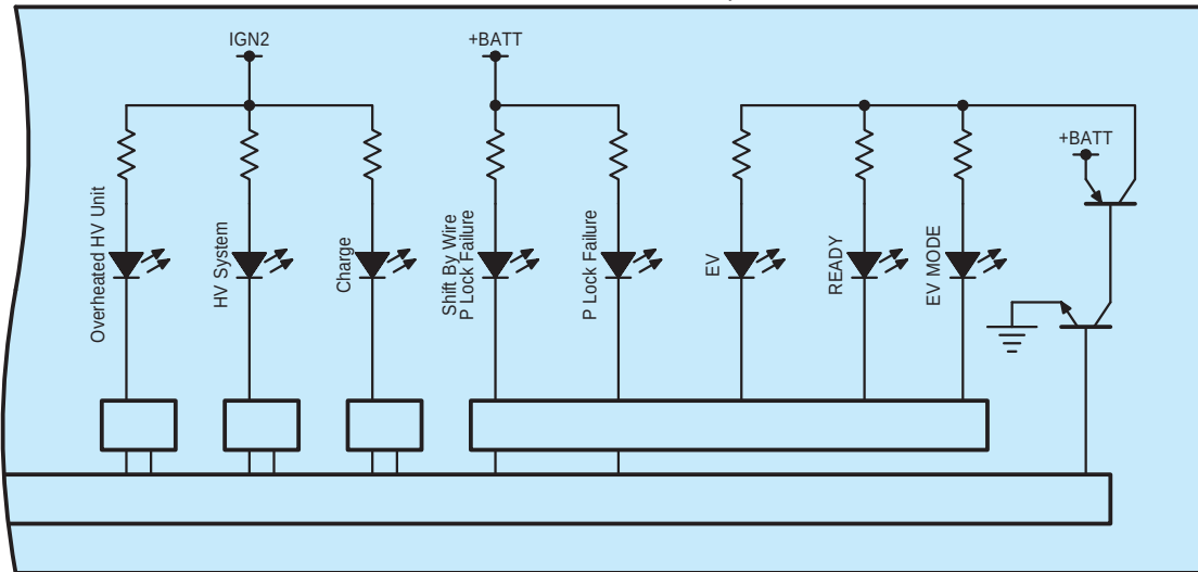
L27(A) Combination Meter Assembly
