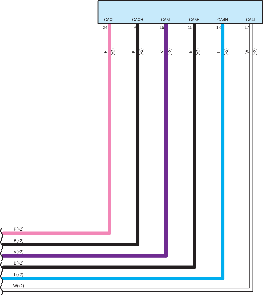
L192 Network Gateway ECU
