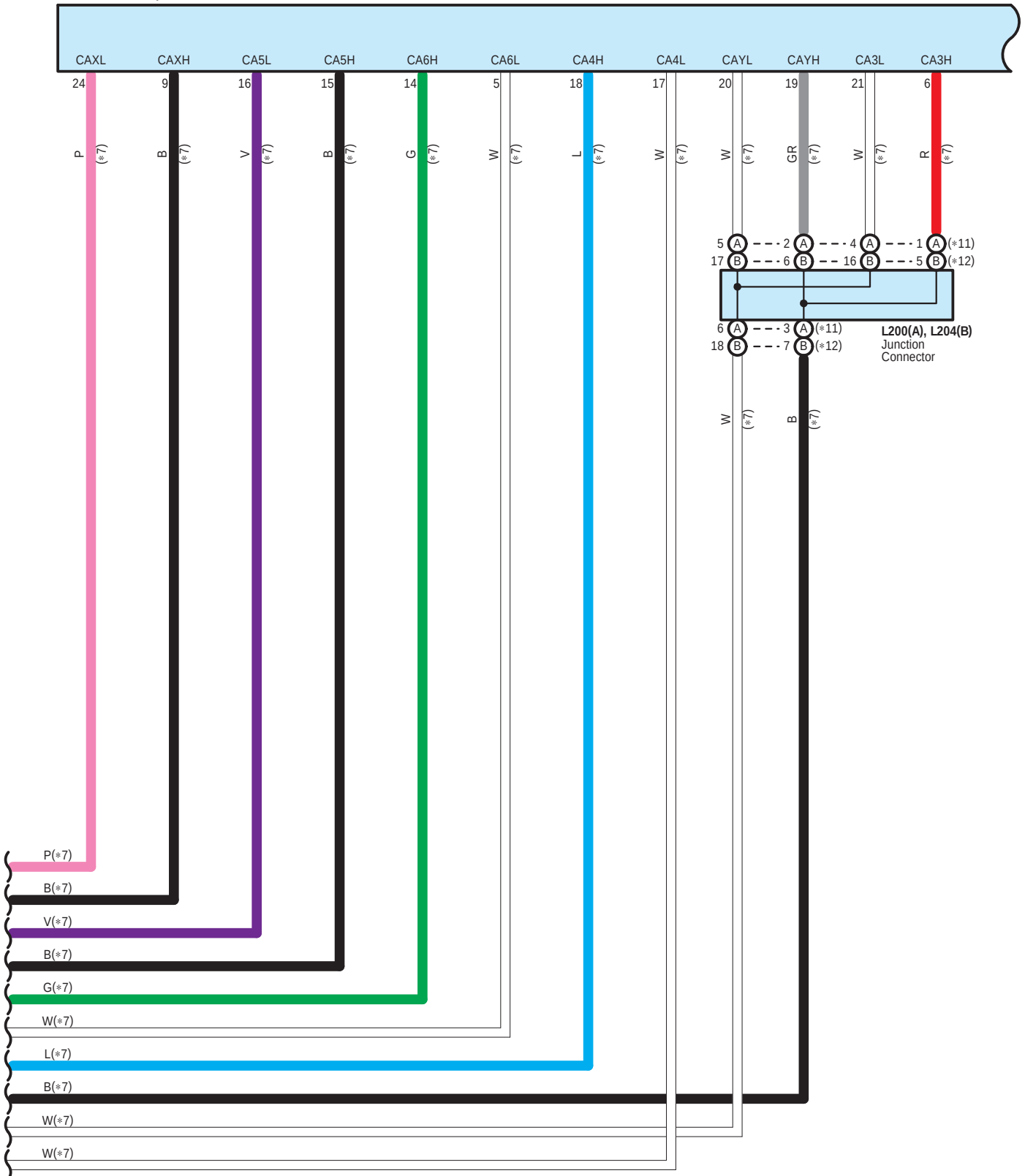
L192 Network Gateway ECU
