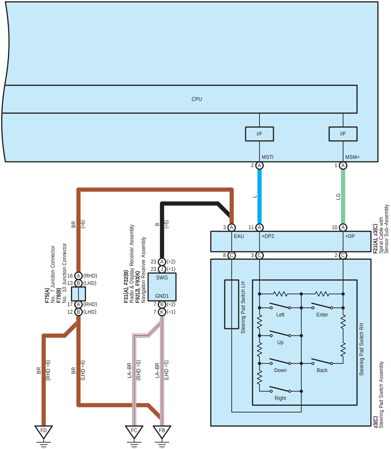
F6(A), F7(B) Combination Meter Assembly
