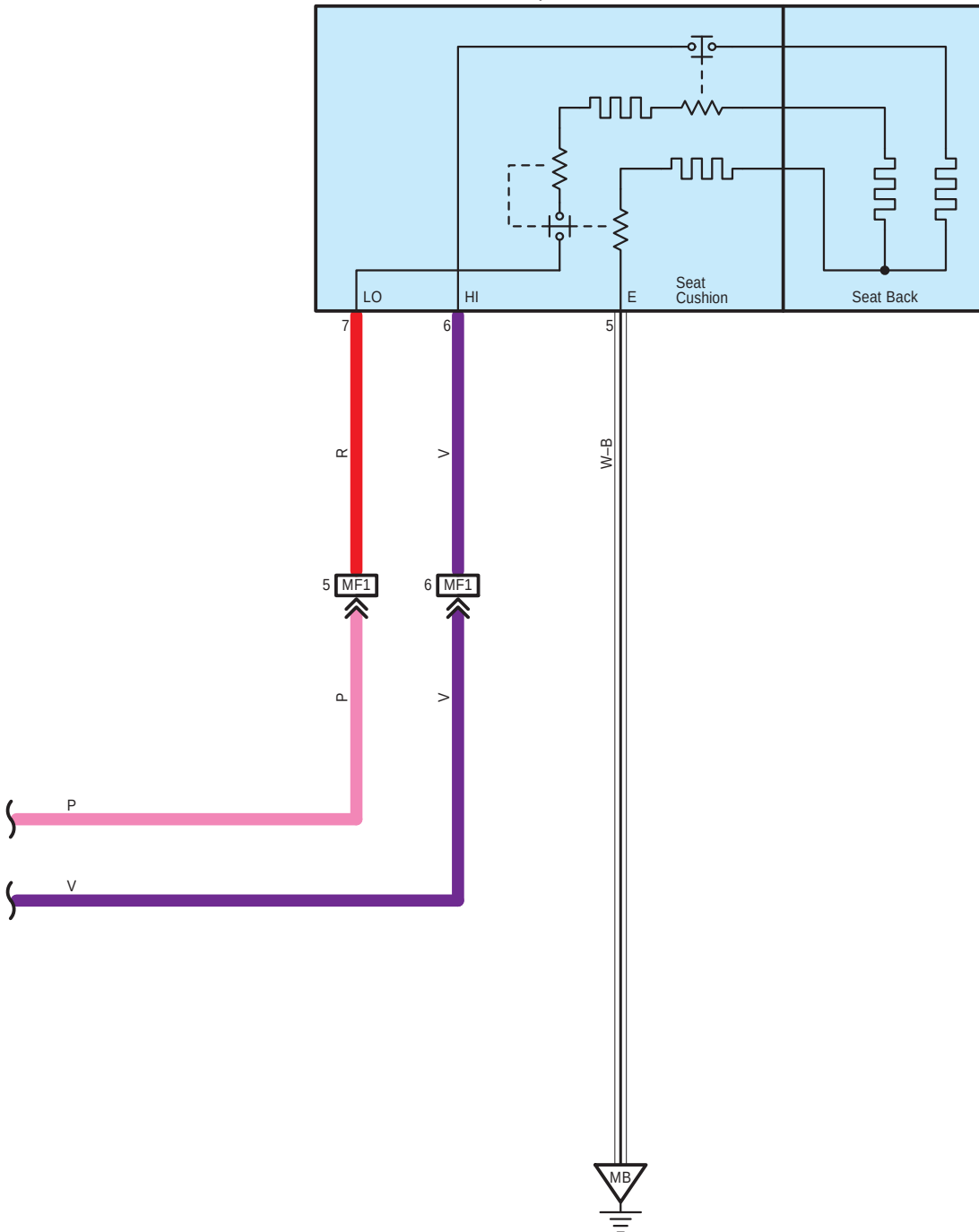
M82 Front Seat Cushion Heater Assembly LH
