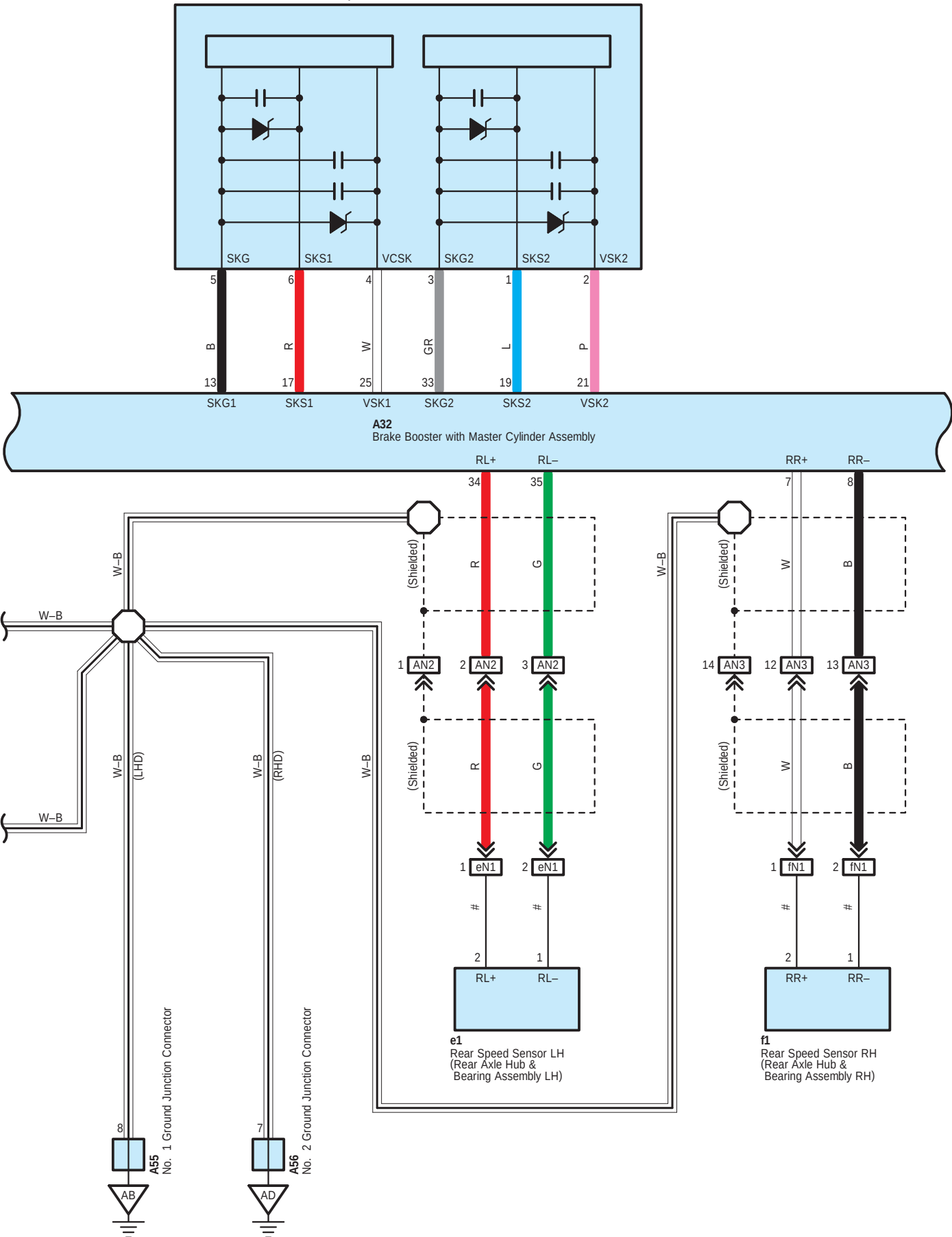
A36 Brake Pedal Stroke Sensor Assembly
