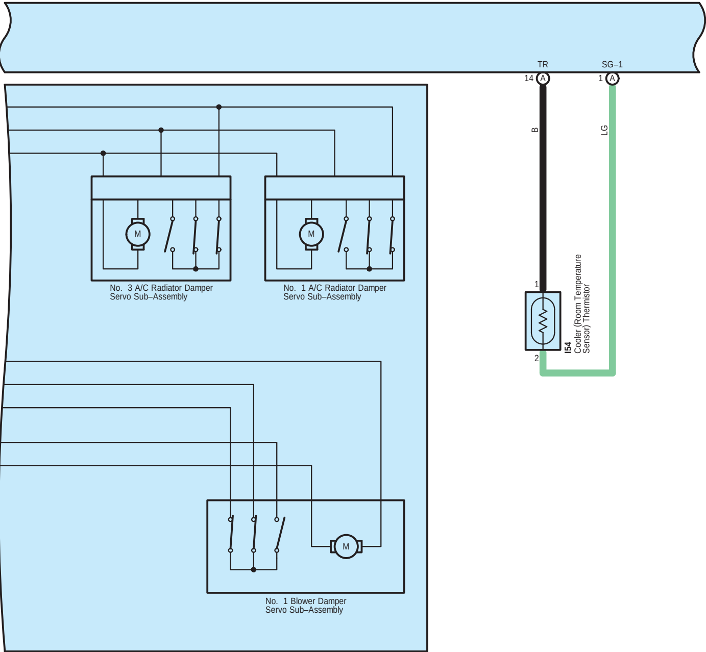
z1(C) A/C Harness Assembly
