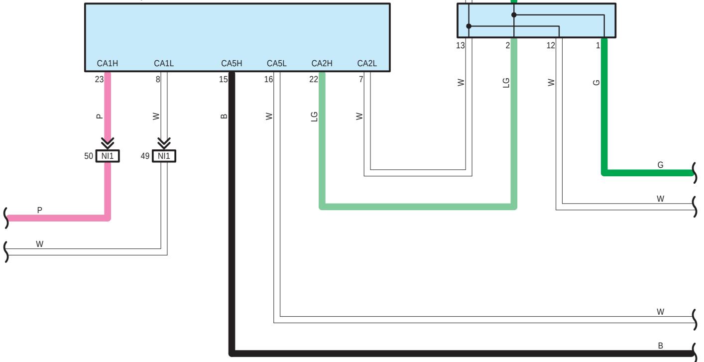
I62 Network Gateway ECU
