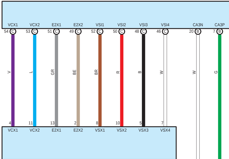
I51 Shift Lock Control Unit Assembly
