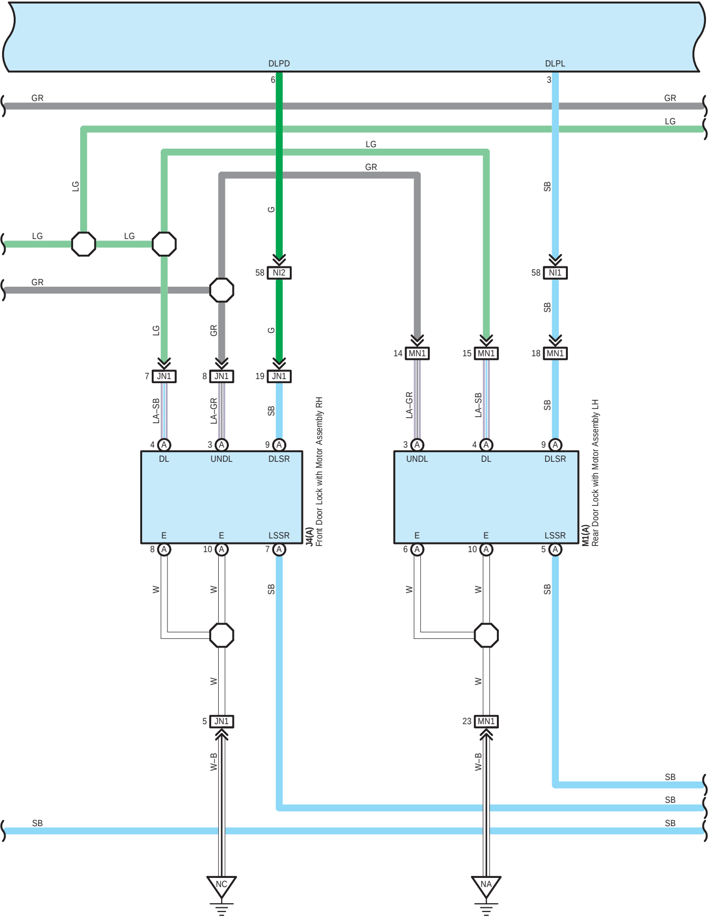
I16 Double Lock Door Control Relay Assembly
