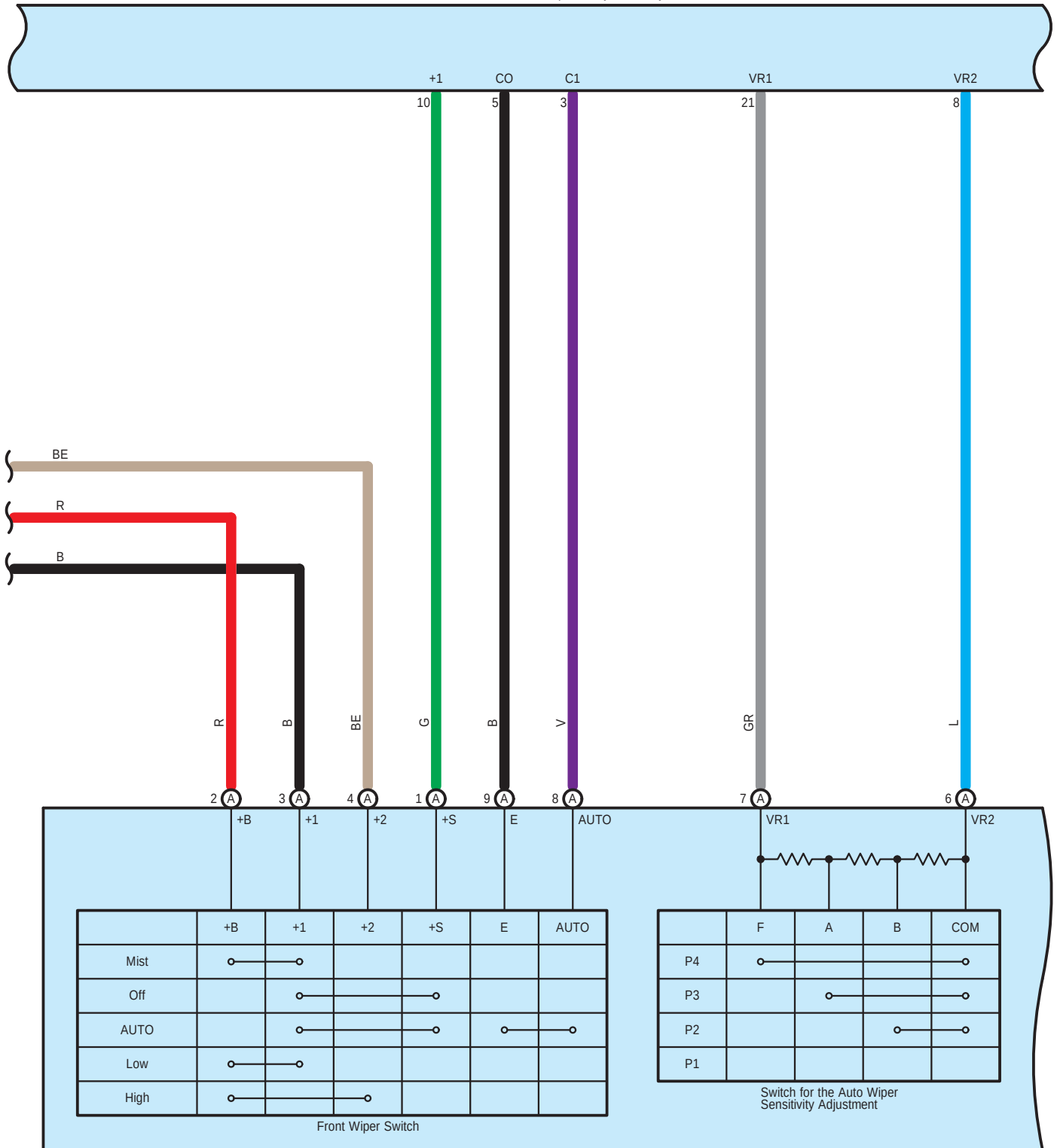
I68(A), I69(B) Windshield Wiper Switch Assembly
