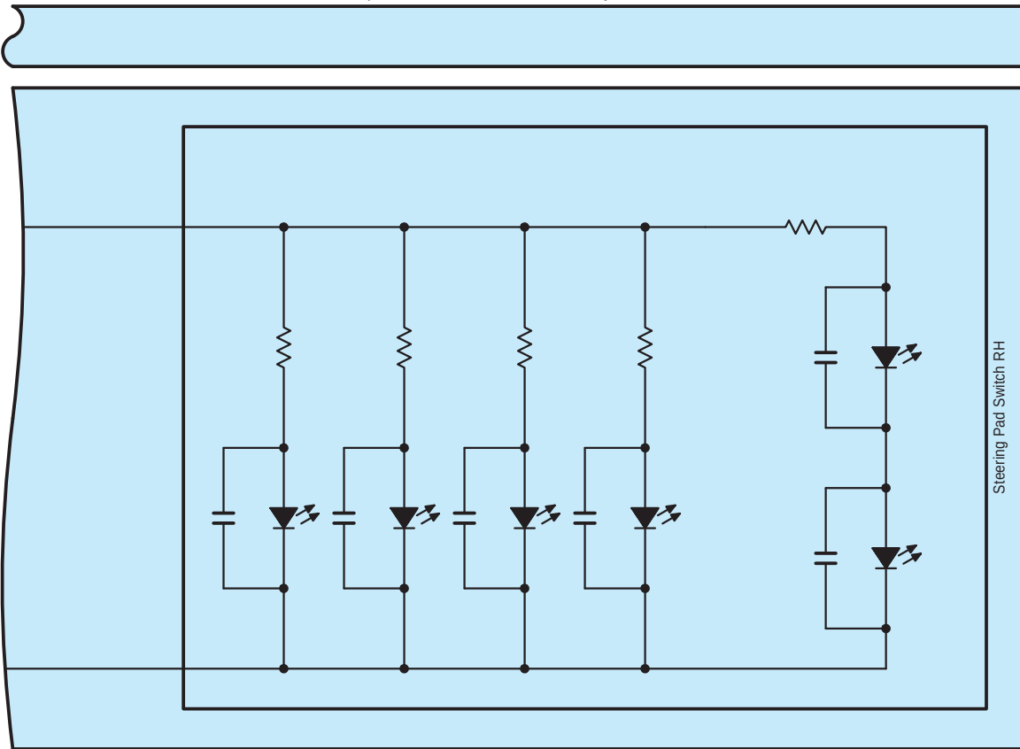
z3(D) Steering Pad Switch Assembly
