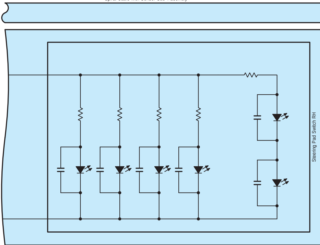
z3(D) Steering Pad Switch Assembly
