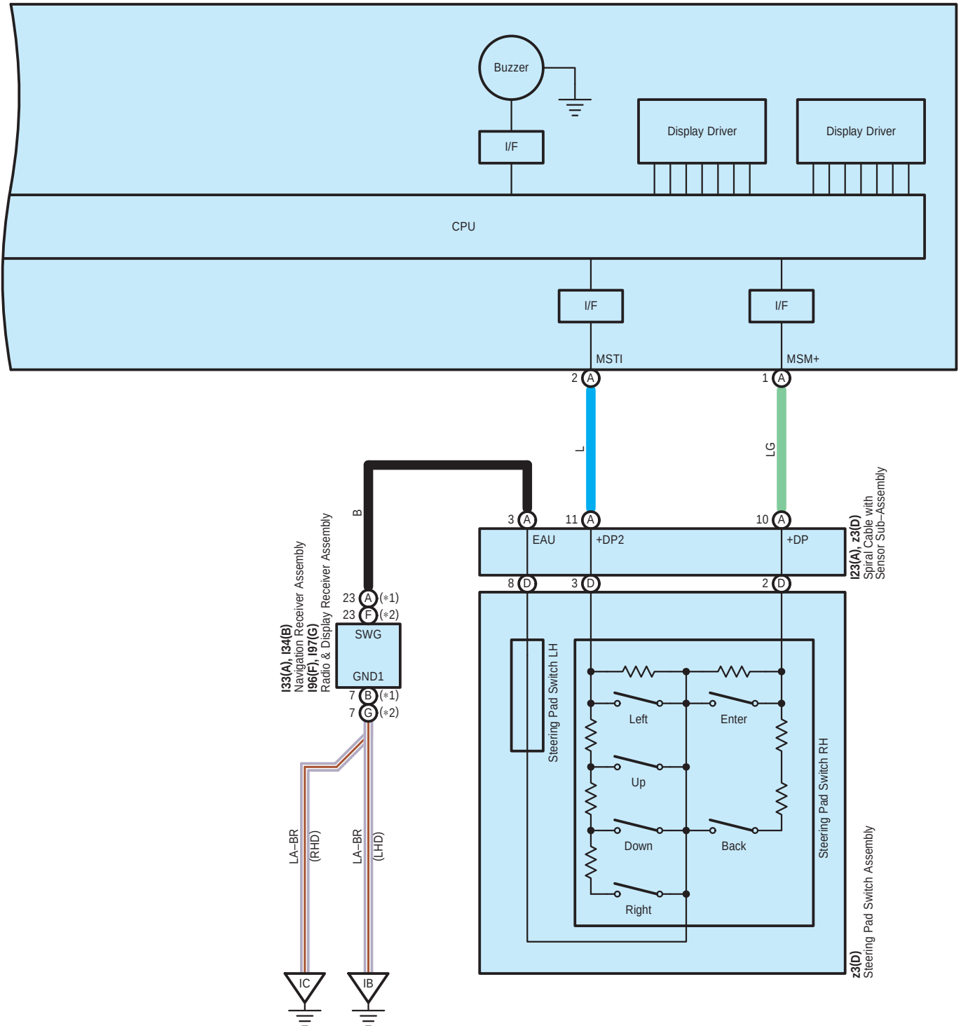
16(A), 17(B) Combination Meter Assembly
