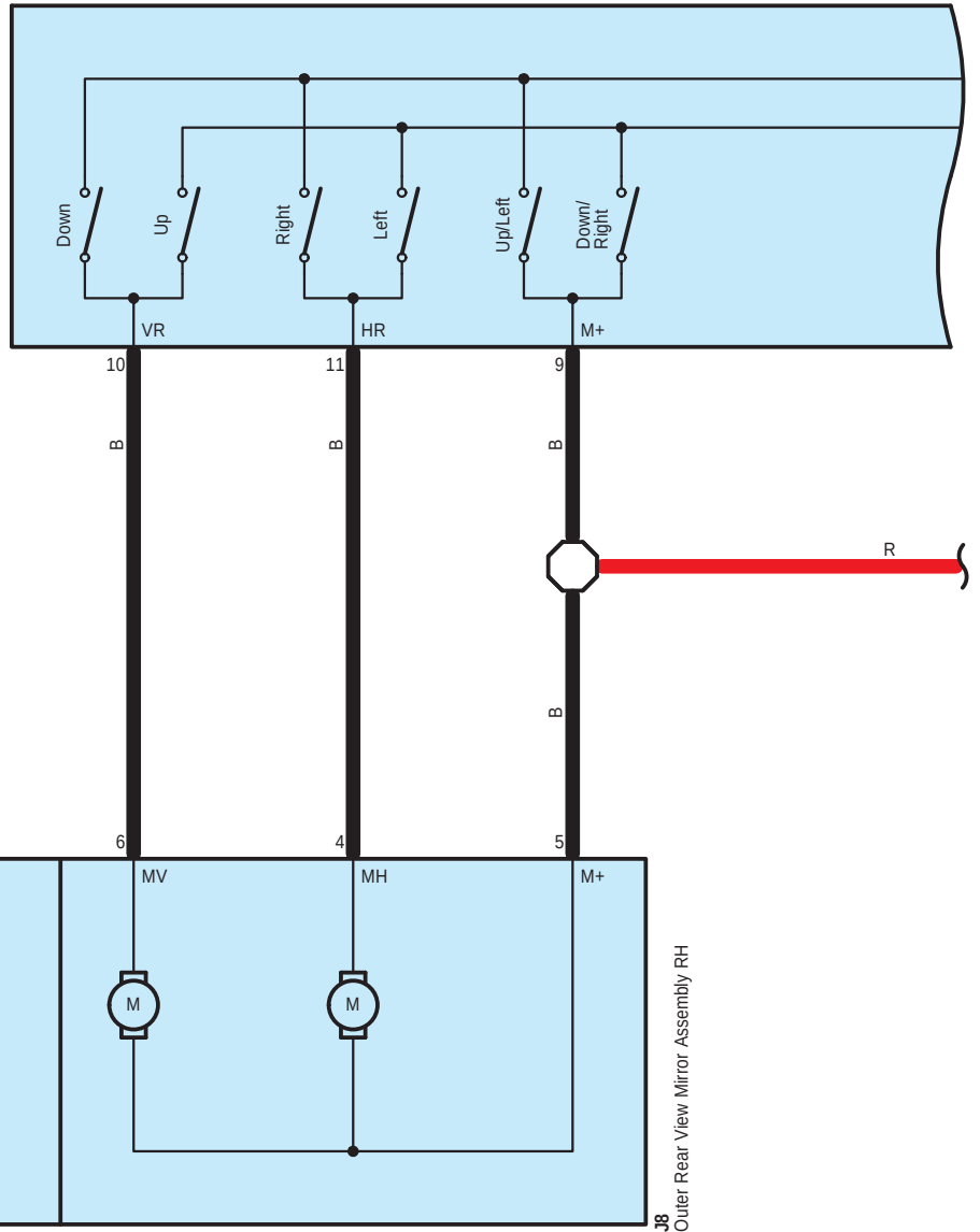
J11 Outer Mirror Switch Assembly
