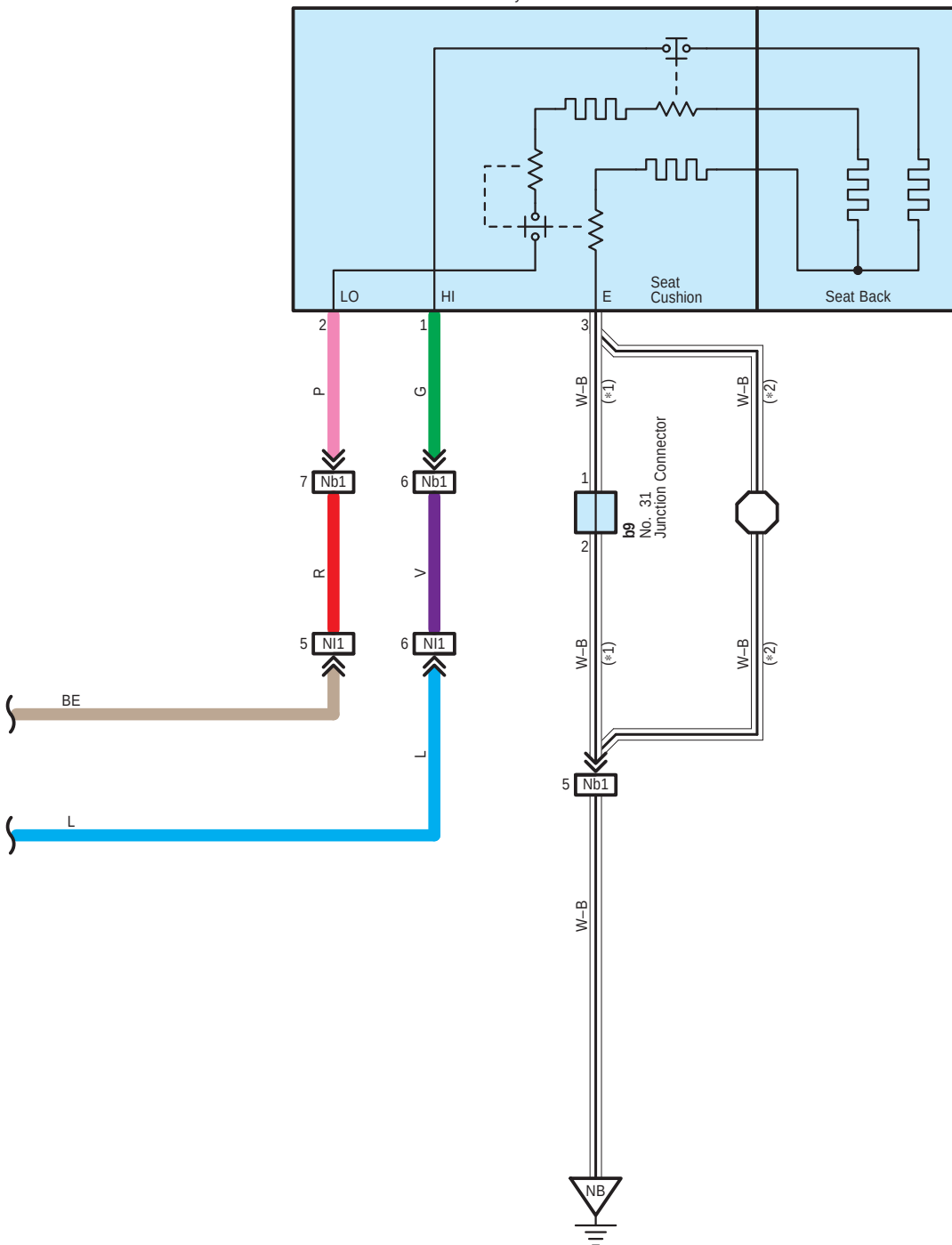
b6 Front Seat Cushion Heater Assembly LH
