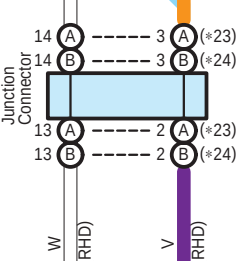
E77(A), E115(B) Junction Connector
